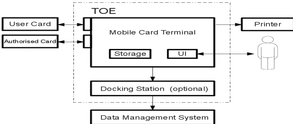
Figure 1: TOE demarcation
