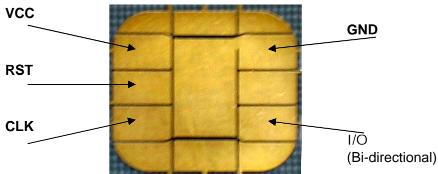
Figure 4: Example of contact plate used to provide electrical communication with the cryptographic module. Contacts that are not identified do not carry any signals and are either grounded or left not connected.
