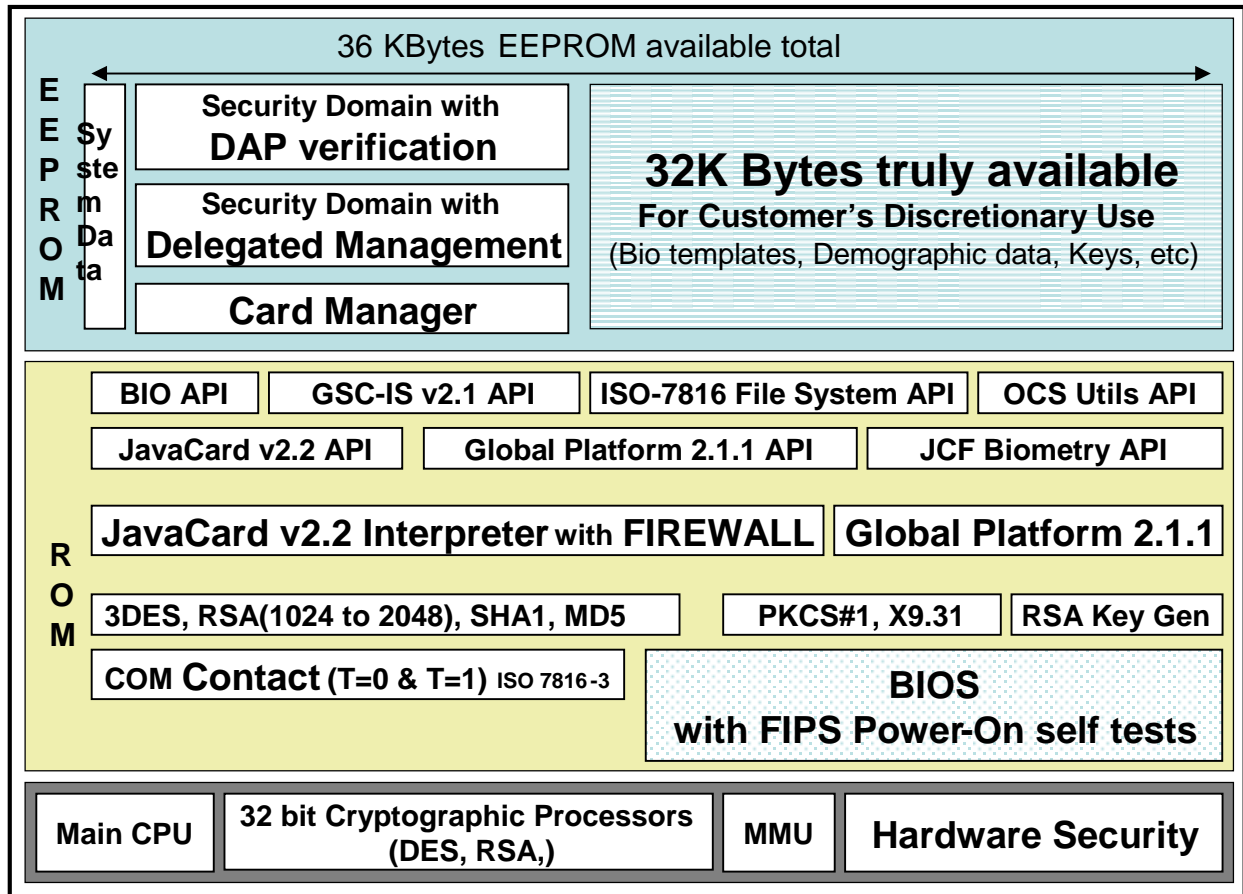
Figure 3: Logical Block Diagram of the Oberthur ID-One Cosmo 32 v5
