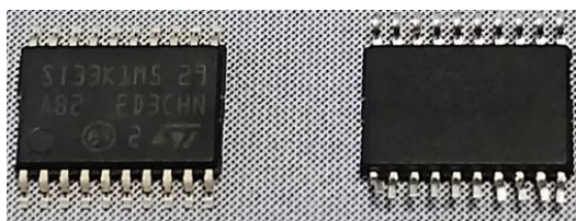
Figure 3 – TSSOP20 Package
