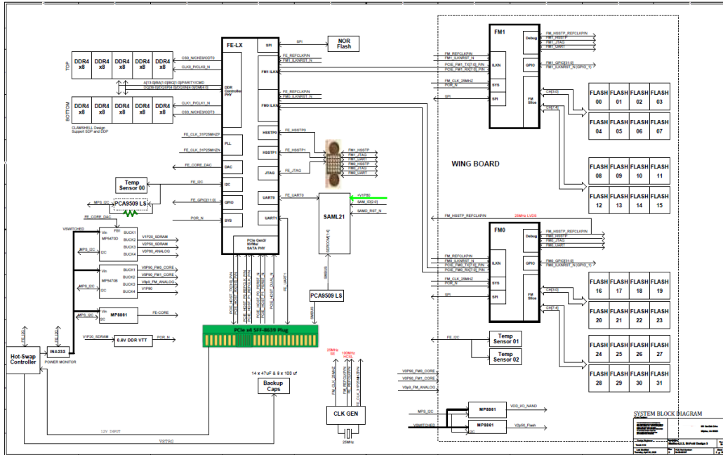
Figure 3: Ultrastar DC SN540/ZN540 Block Diagram
