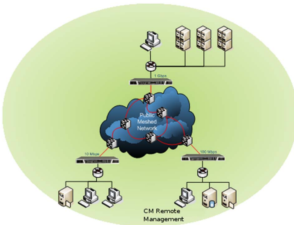
Figure 5 - Meshed Configuration
