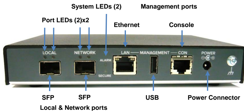
Figure 19 - Rear View of the CN4020 [O] and CN4020 [Y] Encryptors
