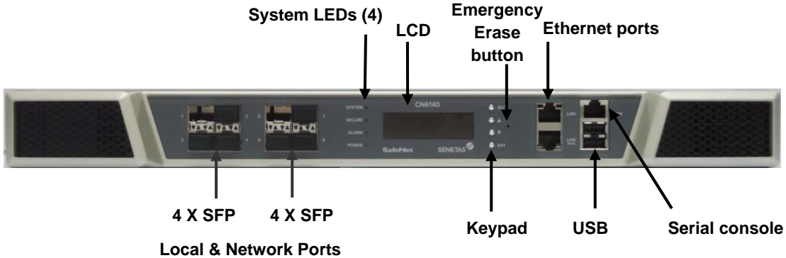
Figure 9 - Front View of the CN6140 [Y] Encryptor
