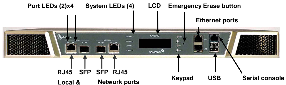
Figure 12 - Front View of the CN6010 [Y] Encryptor
