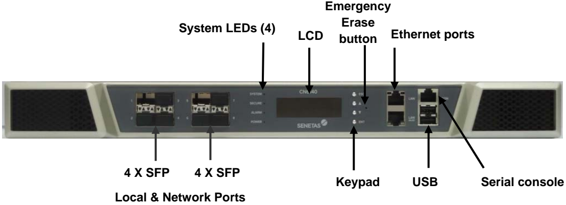
Figure 10 - Front View of the CN6140 [0] Encryptor
