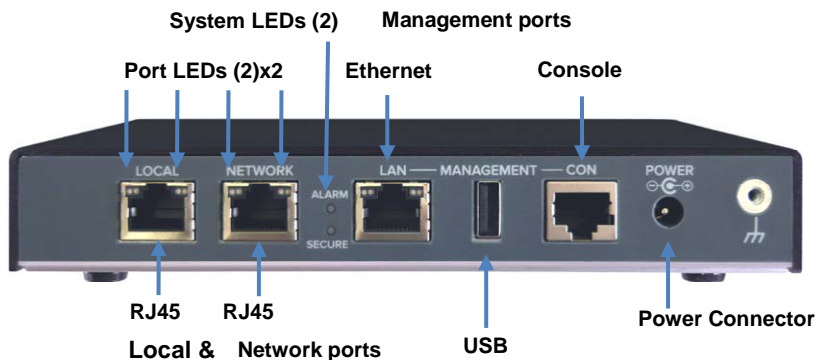
Figure 22 - Rear View of the CN4010 [O] and CN4010 [Y] Encryptors
