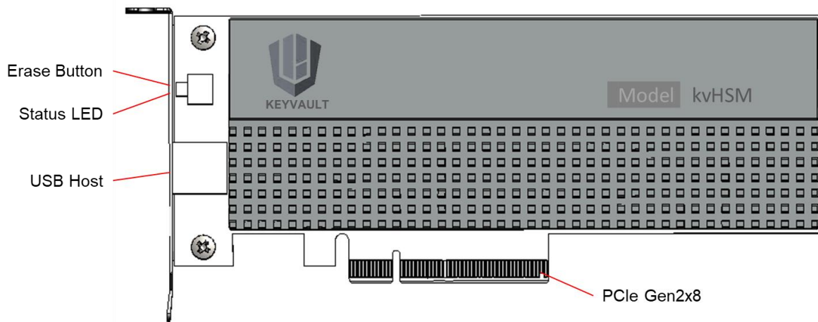
Figure 8 – Physical ports
