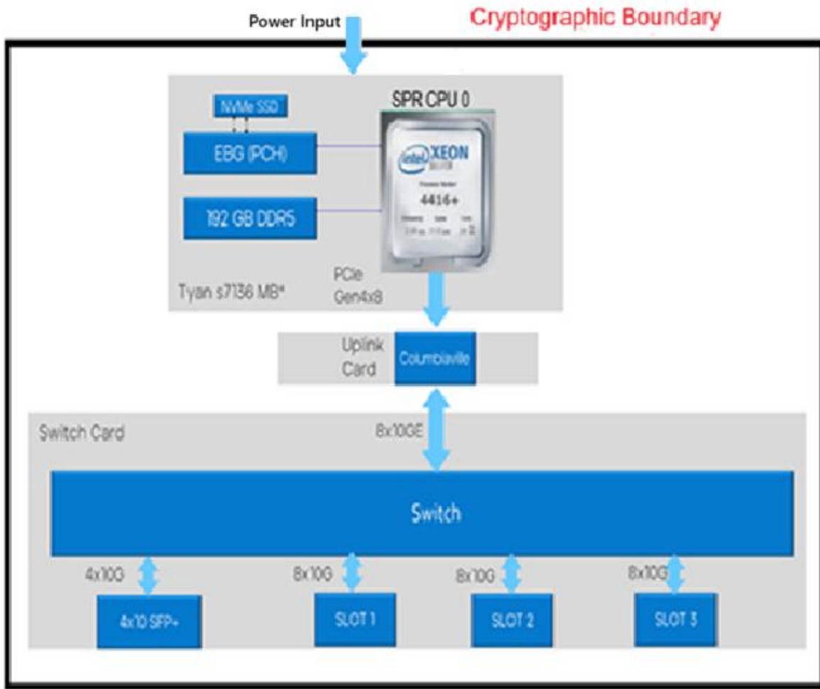
Figure 3: Block Diagram of the Trellix Intrusion Prevention System Sensor NS7600
