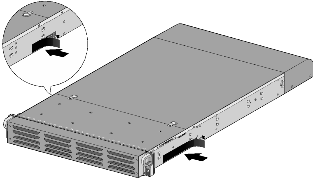
Figure 12 - Apple Tamper-Evident Seals on Vent Overlays
