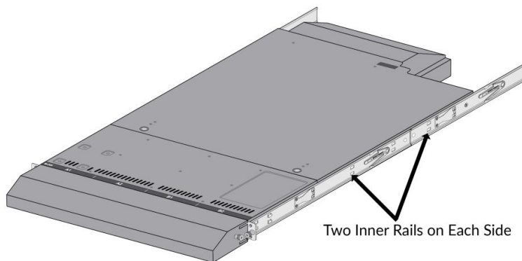
Figure 11 – M-200: Inner Rack Mount Rail Brackets
