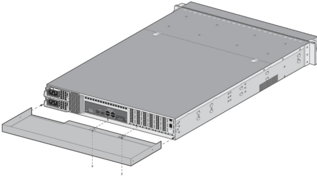
Figure 10 - Install Rear Opacity Shield Tray
