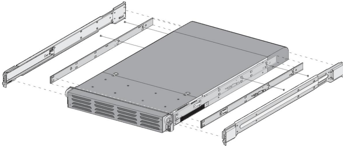
Figure 14 - Install Rail Kit
