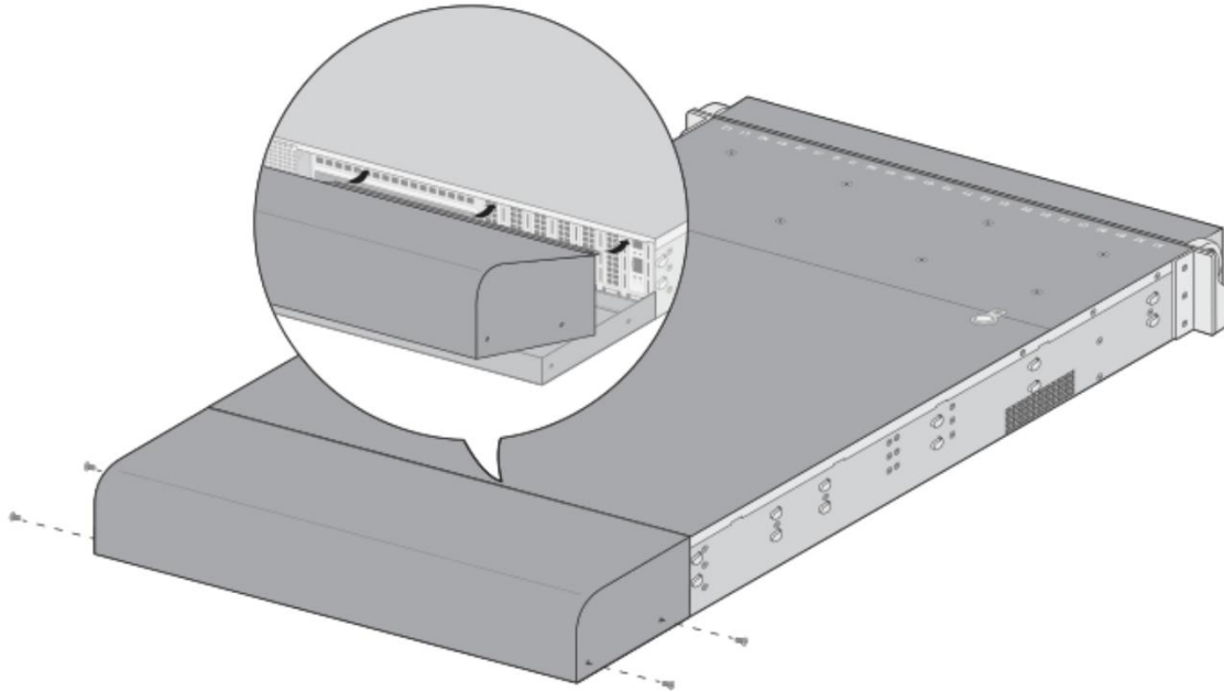
Figure 11 - Install Rear Opacity Shield
