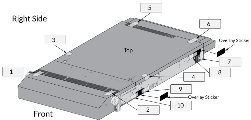
Figure 21 – WF-500-B: Tamper Seal Locations (Top and Front)
