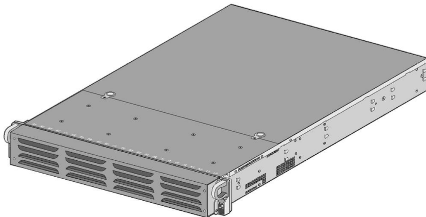
Figure 9 – Front Opacity Shield Installed
