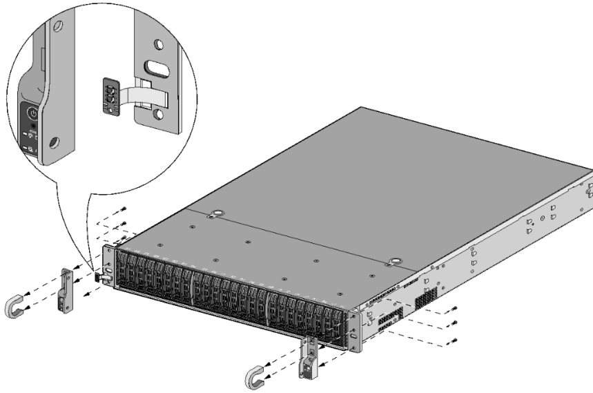
Figure 5 - Remove Front Handles and Modules
