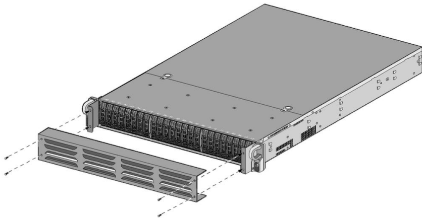
Figure 8 – Install Front Opacity Shield
