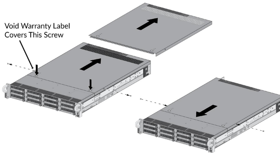
Figure 17 – WF-500-B: Top Cover Replacement
