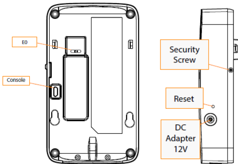
Figure 10 - Aruba IAP-503H Wireless Access Point – Interfaces (Rear and Right Side Views)
