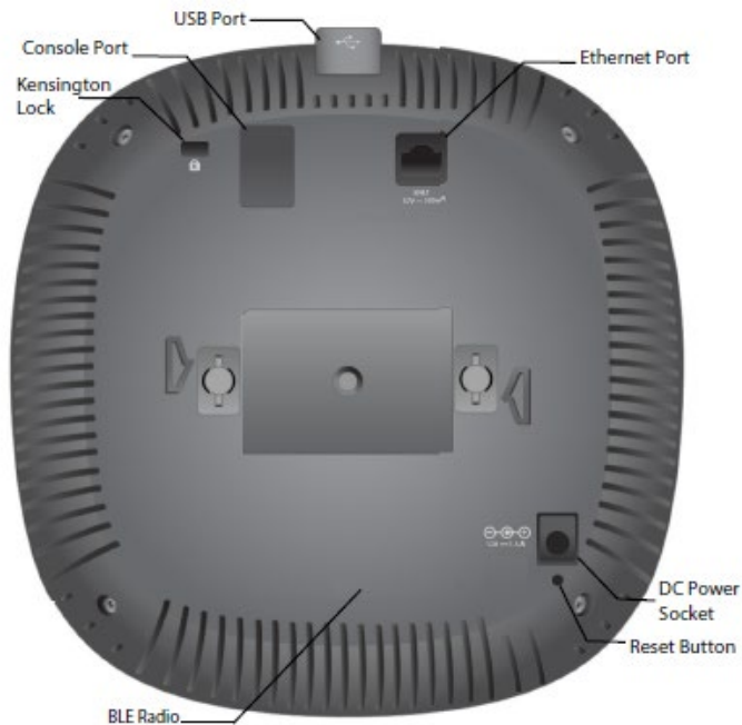
Figure 2 - Aruba IAP-315 Access Point – Interfaces
