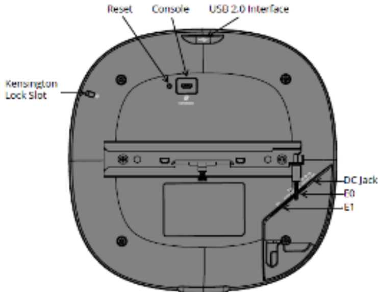
Figure 26 - Aruba IAP-510 Series Wireless Access Point – Interfaces
