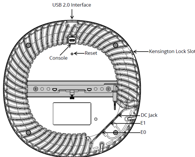
Figure 37 - Aruba IAP-630 Series Wireless Access Point – Interfaces
