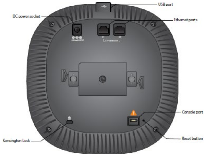
Figure 4 - Aruba IAP-345 Access Point – Interfaces
