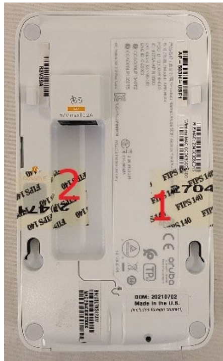
Figure 52 – Rear View of IAP-503H with TELs
