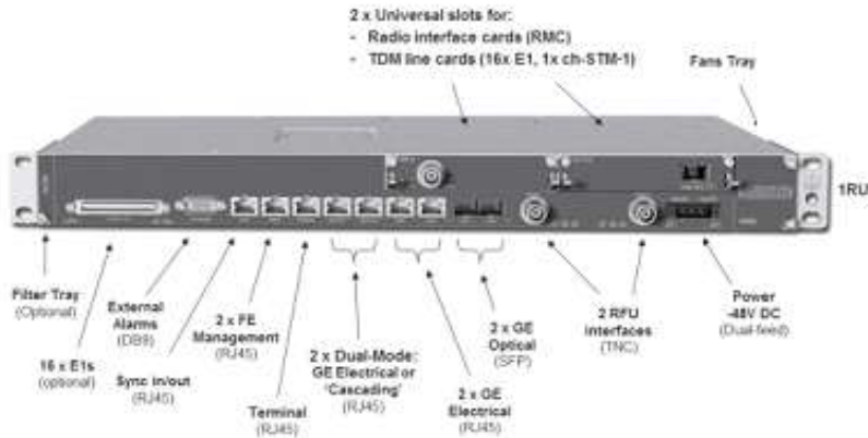
Figure 10 - PTP 820GX Interfaces
