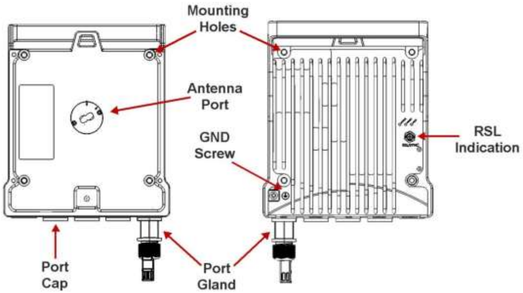
Figure 12 - PTP 820S Interfaces (Front and Back)
