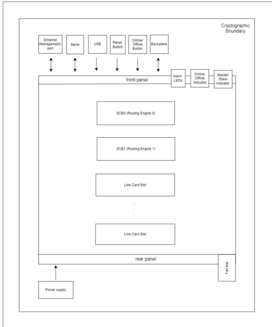
Figure 2: Block Diagram
