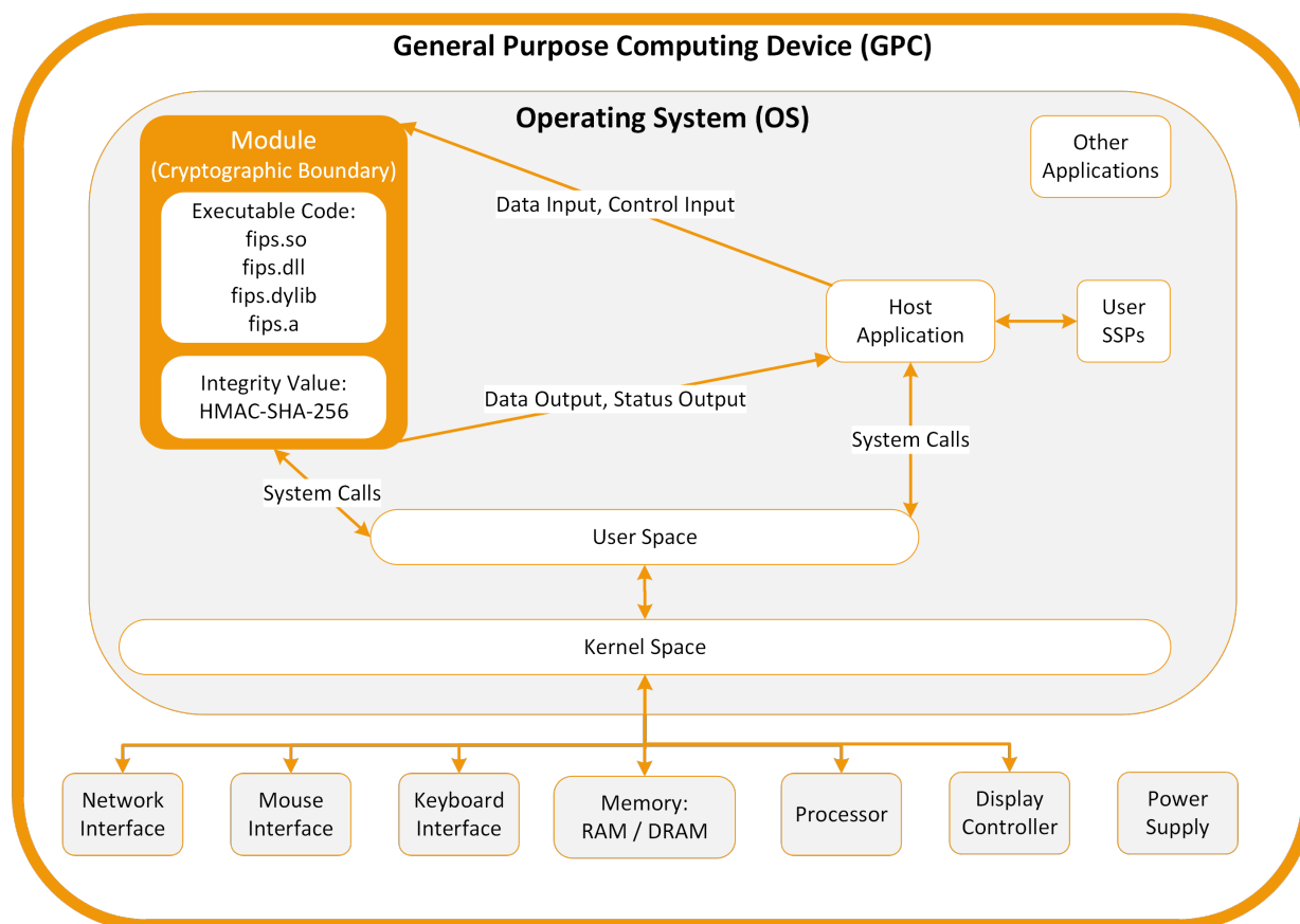
Figure 1: Block Diagram
