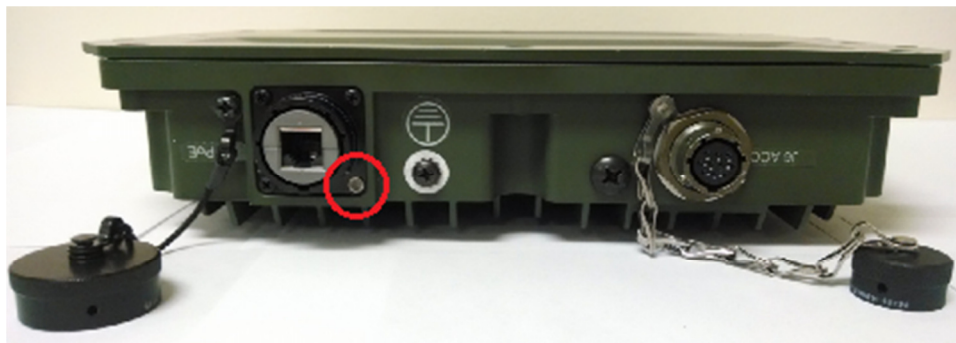
Figure 4 – Tamper-Evident Pin Location for RF-7800W
