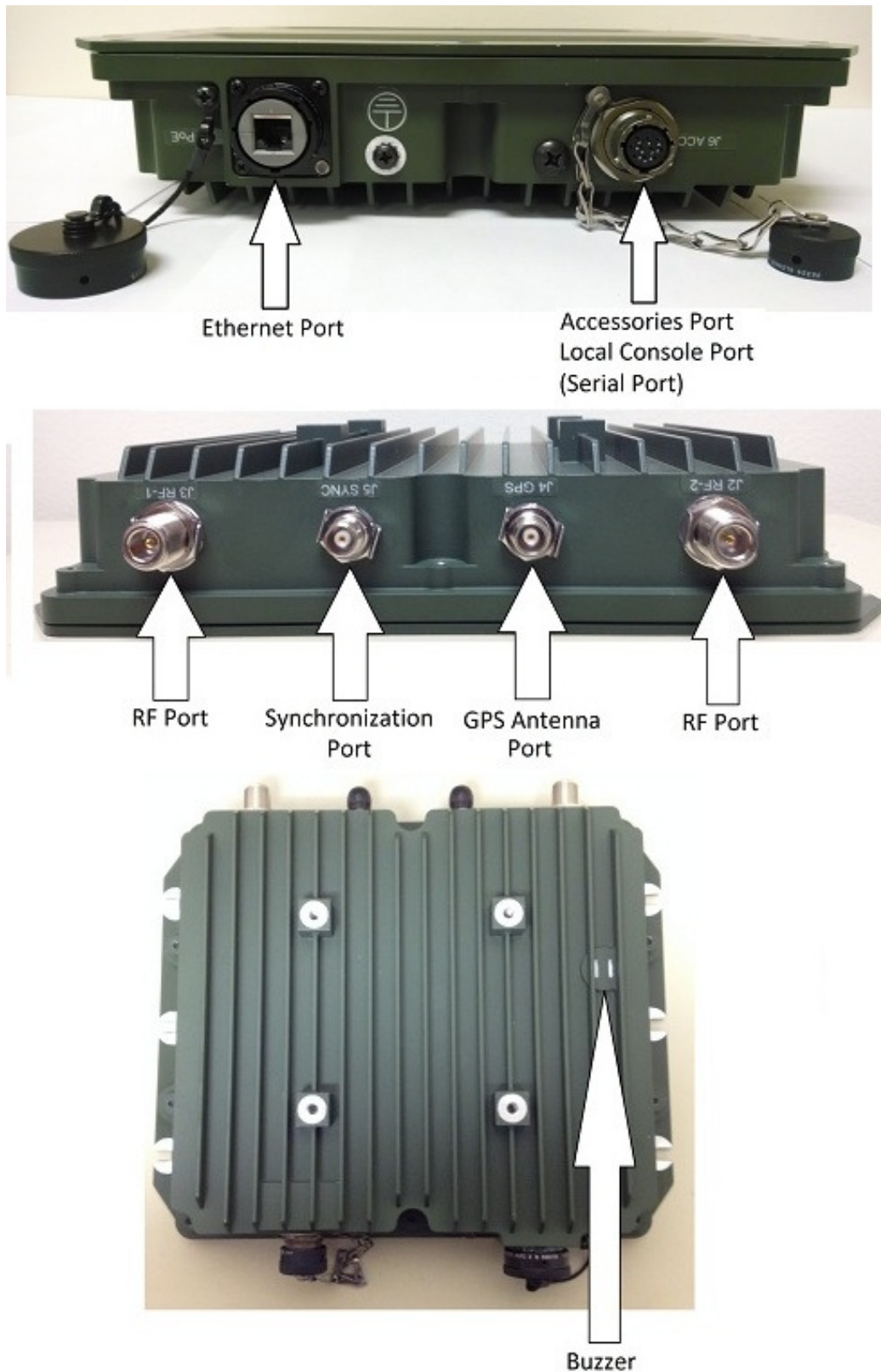
Figure 2 – Location of Physical Interfaces
