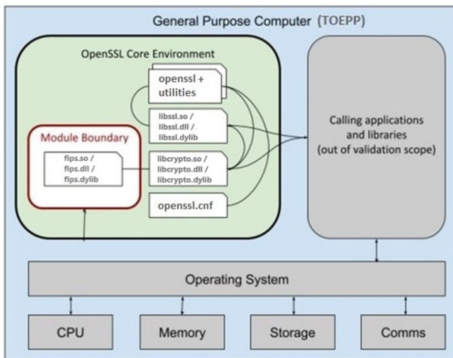
Figure 1: AWS OpenSSL FIPS Module (based on the OpenSSL FIPS Provider) Block Diagram
