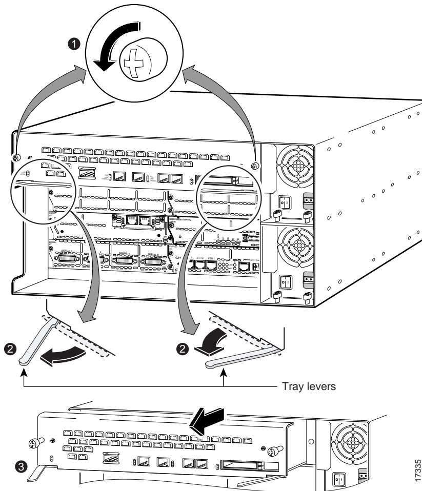
Figure 5 Chassis Removal
