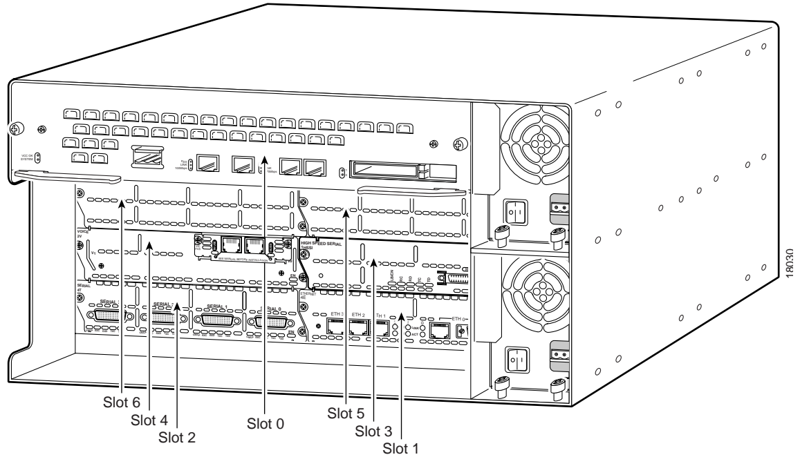
Figure 2 Physical Interfaces
