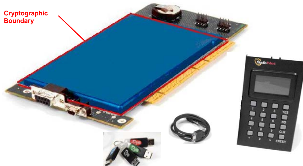
Figure 2-1. Luna PCI Cryptographic Module with PED and iKeys
