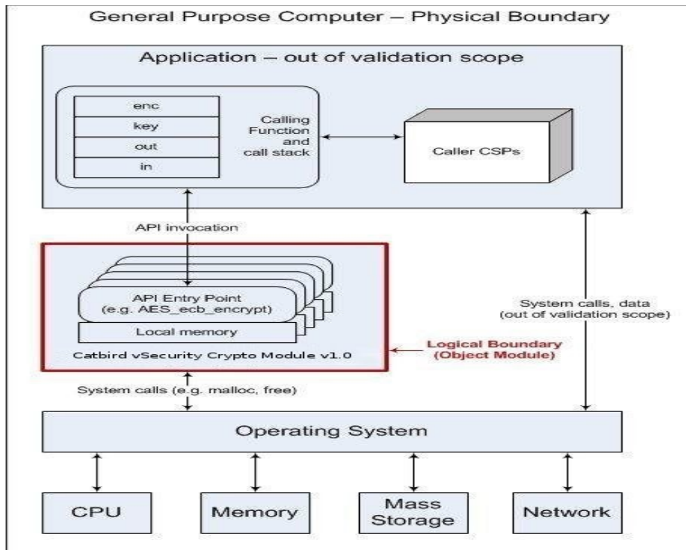
Block Diagram
