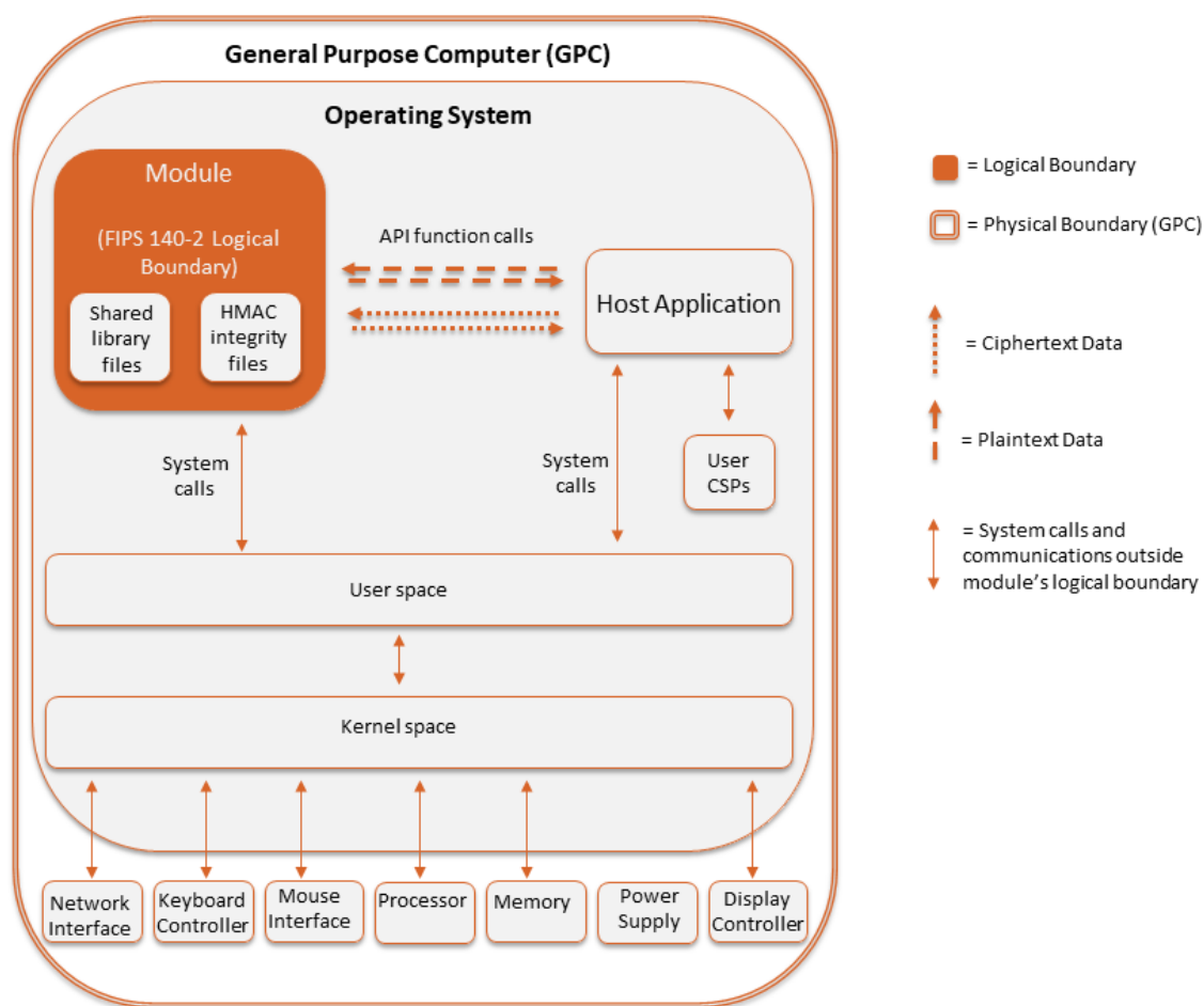
Figure 1 – Module Boundary and Interfaces Diagram
