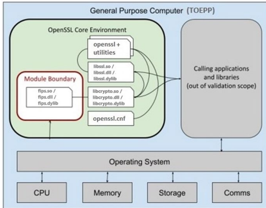
Figure 1: Philips FIPS Provider based on the OpenSSL FIPS Provider Block Diagram
