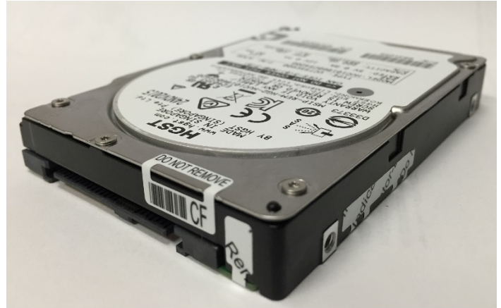
Figure 5: Smaller Tamper-Evident Label Hardware Version (3)
