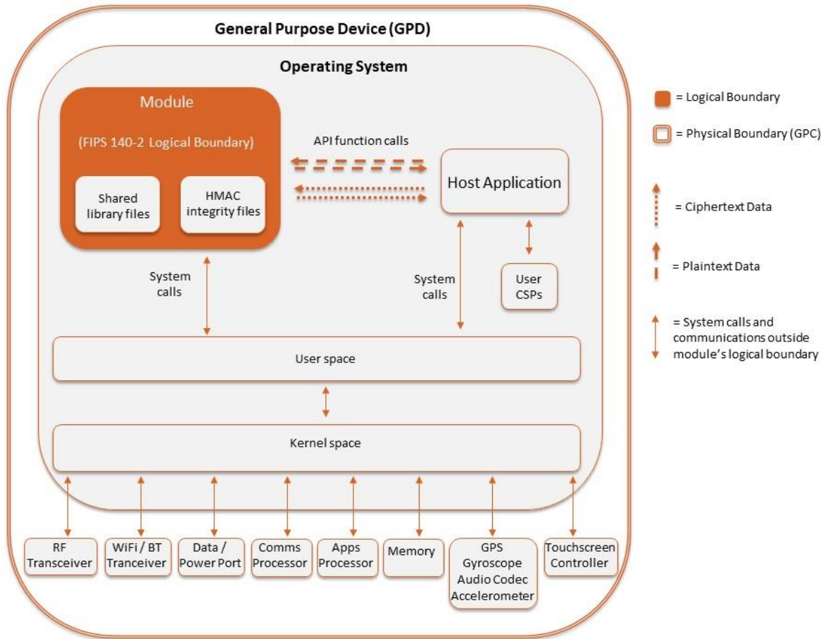
Figure 1 – Module Boundary and Interfaces Diagram
