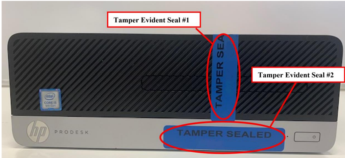
Figure 1 Front
