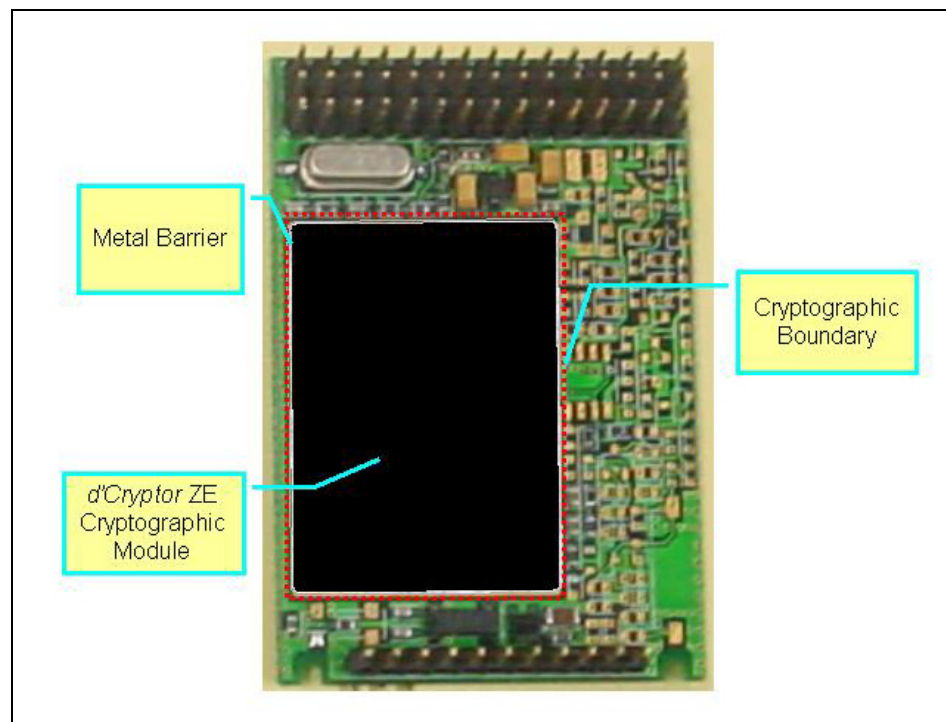
Figure 1. Plan view of d'Cryptor ZE (dotted red line)
