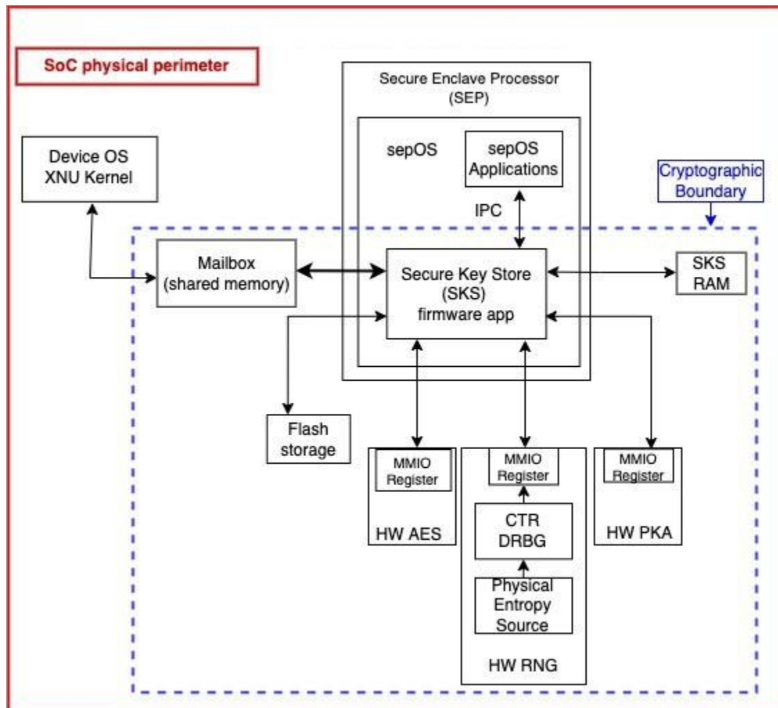
Figure 1: Block Diagram
