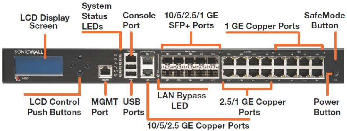
Figure 8 - NS a 9250/NS a 9450/NS a 9650 Front Panel
