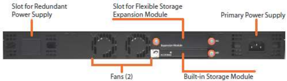
NS a 2650/NS a 3650 Back Panel
