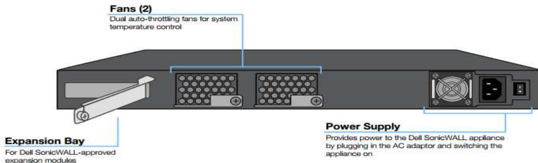
Figure 6 – NS a 6600 Back Panel
