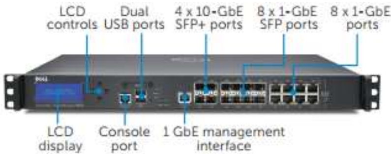
Figure 3– Super Massive Front Panel SM9200/SM 9400/SM 9600
