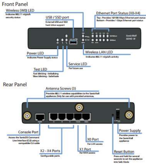
Figure 2 – SOHOW Physical Ports
