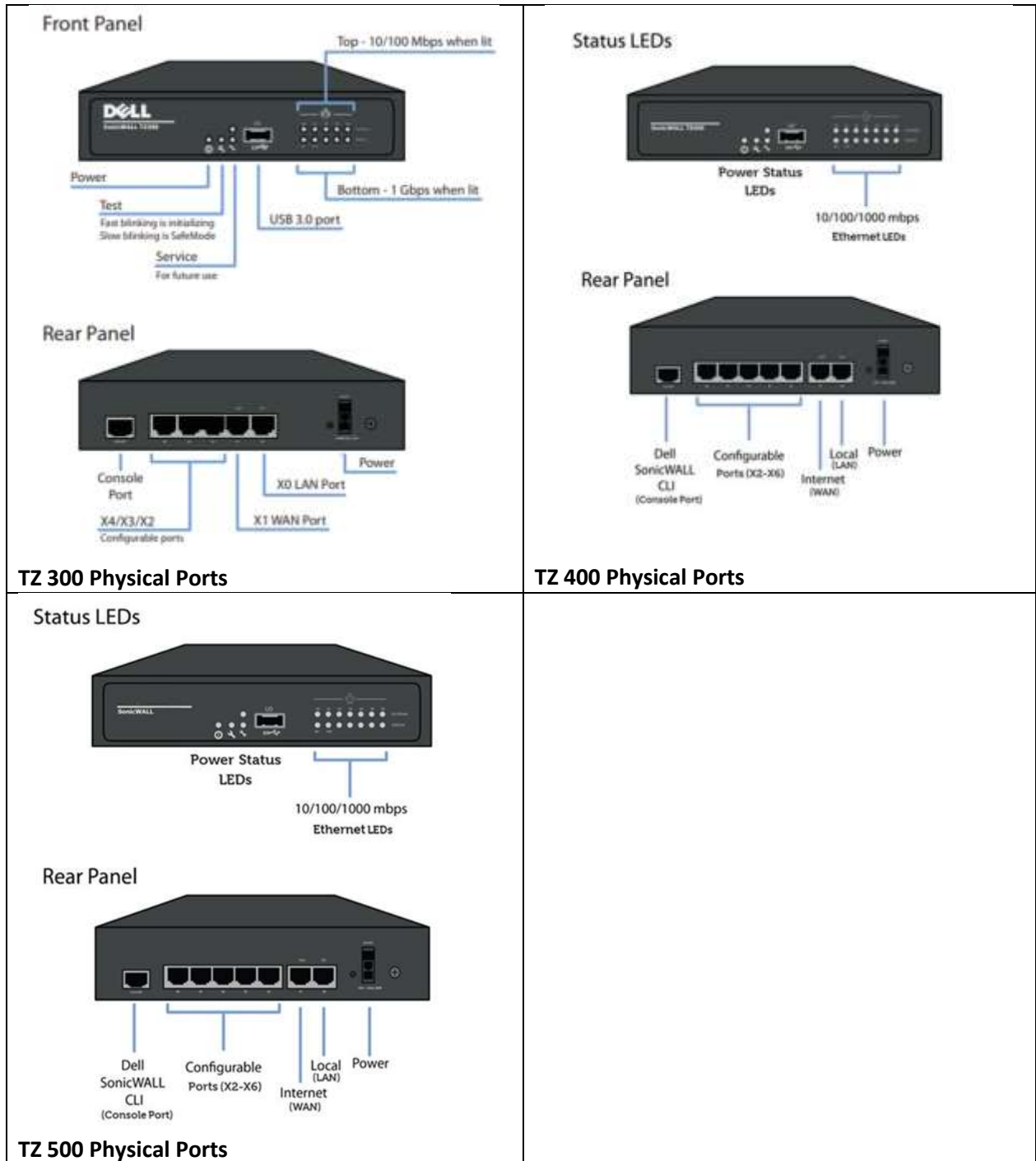
Figure 1 – TZ Series Ports
