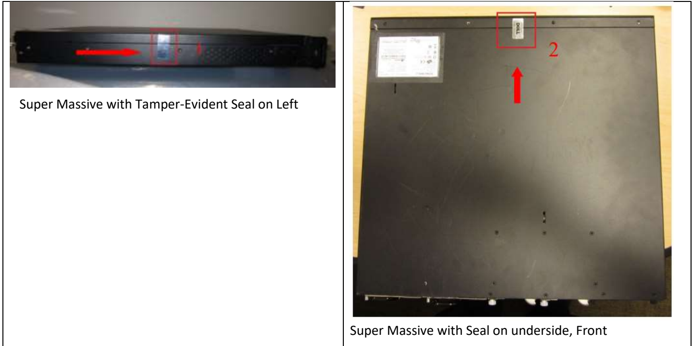
Figure 21: SM 9600/SM 9400/SM 9200
