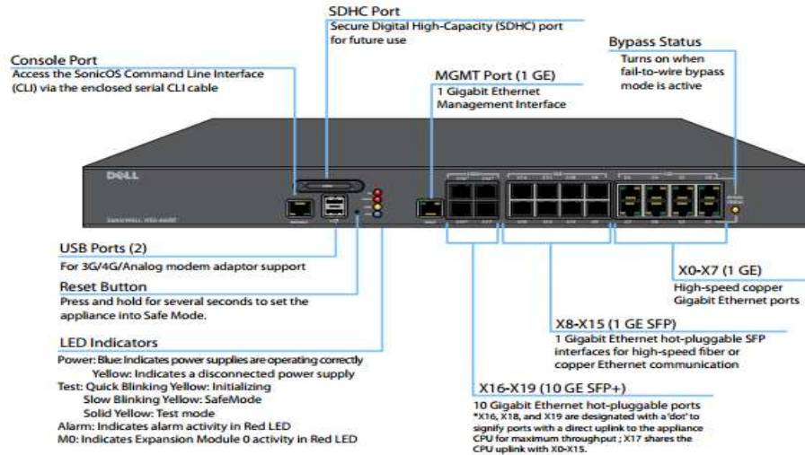
Figure 5 – NS a 6600 Front Panel
