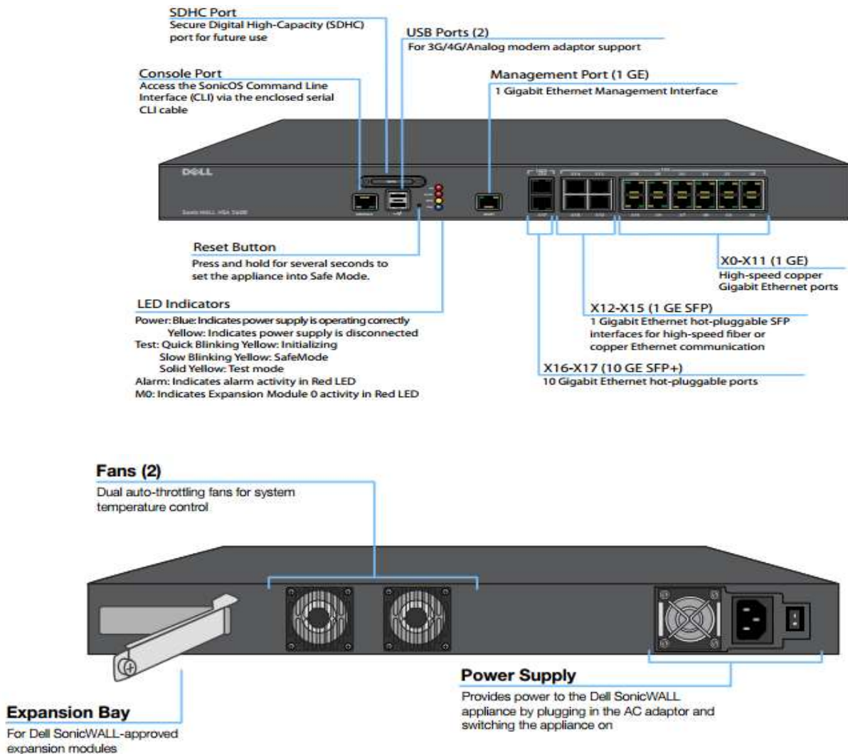
Figure 7 – NS a 5600/NS a 4600/NS a 3600 Front and Back Panel
