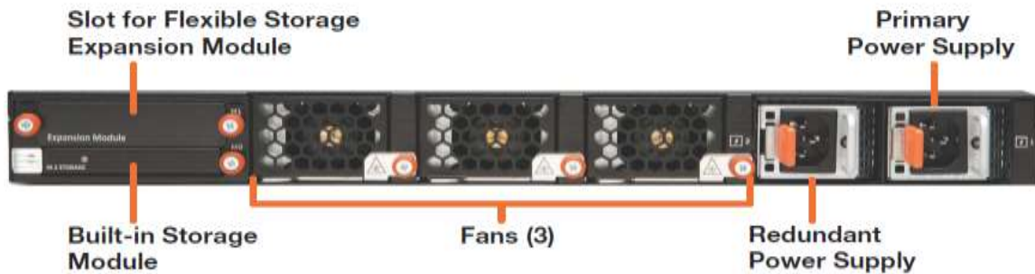
Figure 9 - NS a 9250/NS a 9450/NS a 9650 Back Panel
