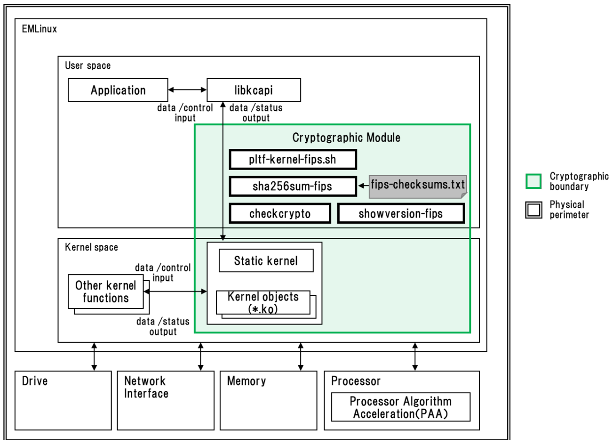
Figure 1: Block Diagram
