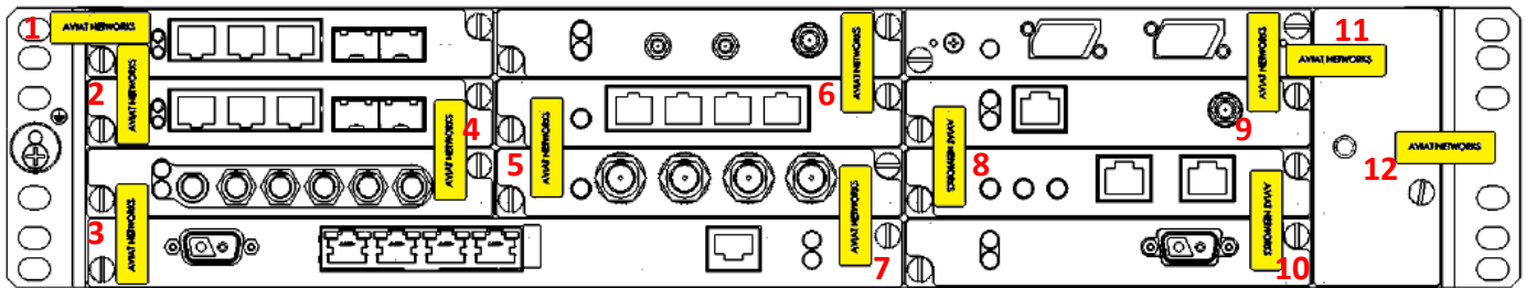
Figure 6 Tamper-Evident Seal Locations (Front)
