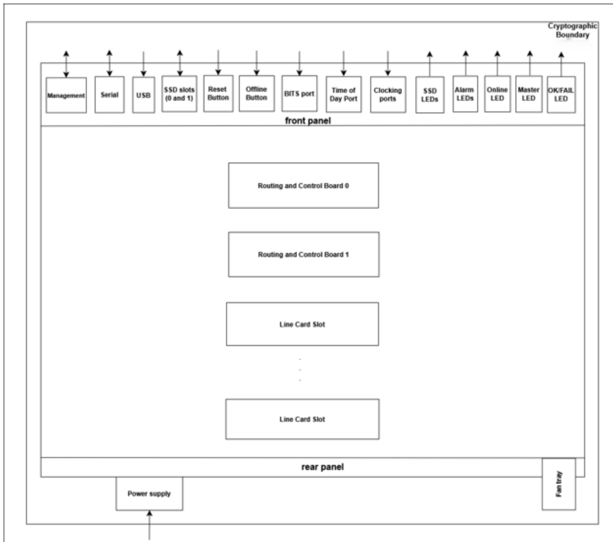
Figure 2 – Block diagram of the MX10003
