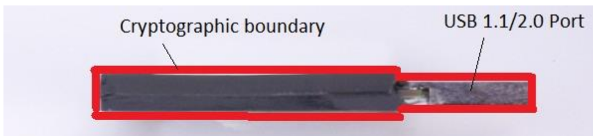
Figure 3 – KDF2000-128G, KDF2000-64G, KDF2000-32G, KVD-SMCF-32G (side)
