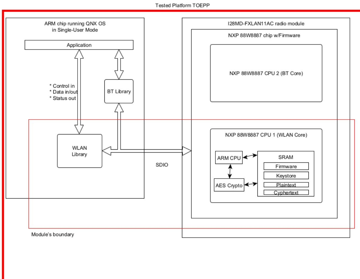
Figure 2: Block Diagram
