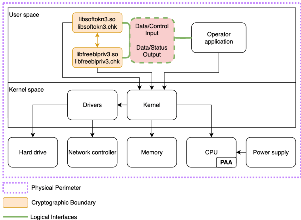
Figure 1: Block Diagram
