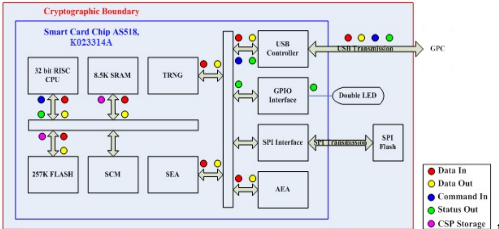
Figure 2. WatchKey ProX USB Token Hardware Block Diagram
