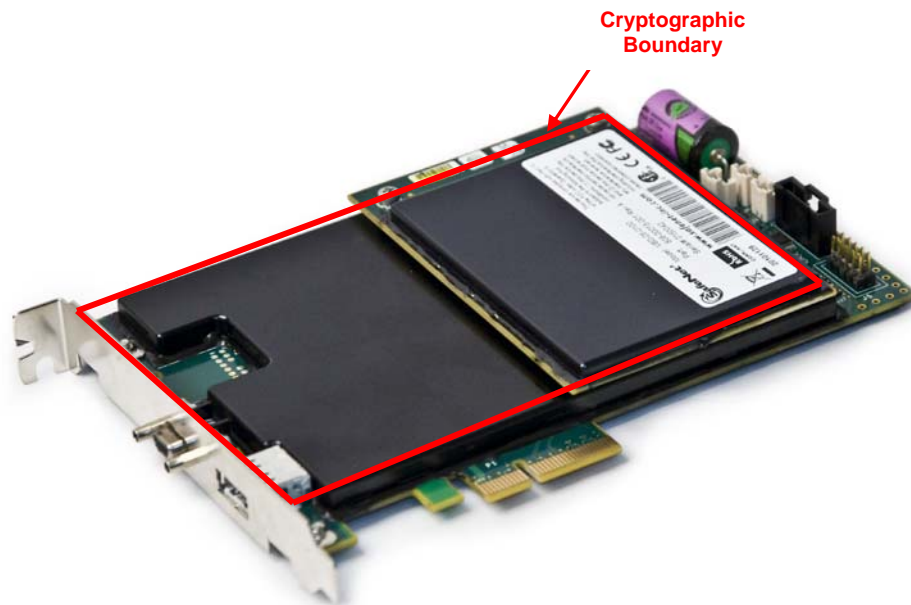
Figure 2-1. Luna PCI-E Cryptographic Module
