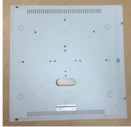
WAB910003-E6 Enclosure (top, connector port)
