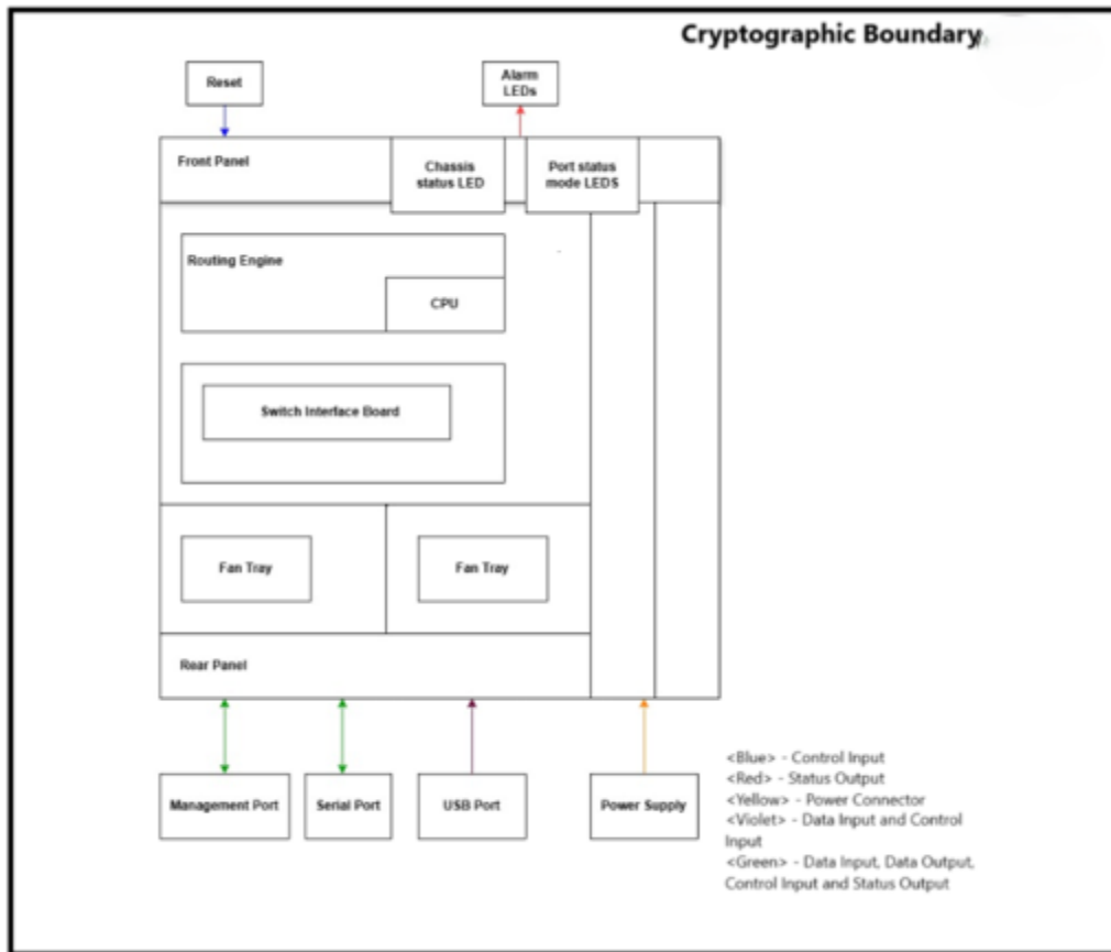
Figure 11 – Block Diagram
