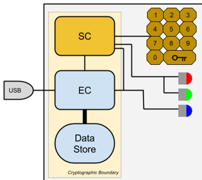
Figure 2: datAshur Pro 3.0 Module Architecture
