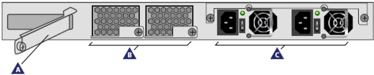
Figure 2 – NSA E7500 Back Panel
