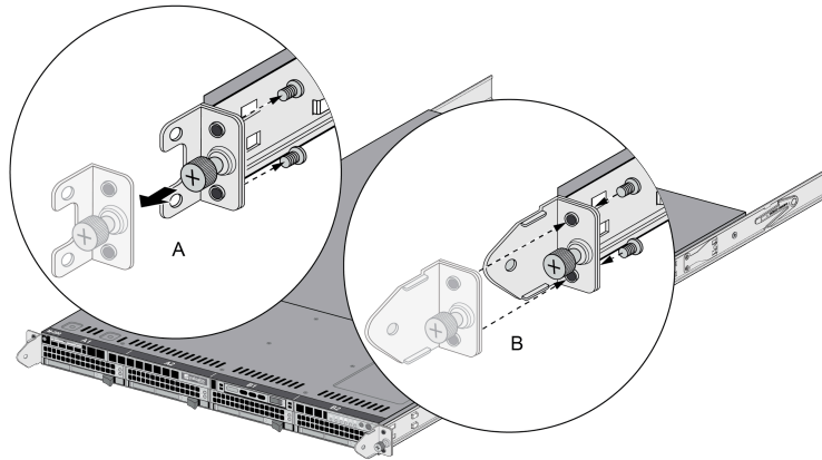
Figure 12 – M-200: Replacing Front Rack-Mount Brackets
