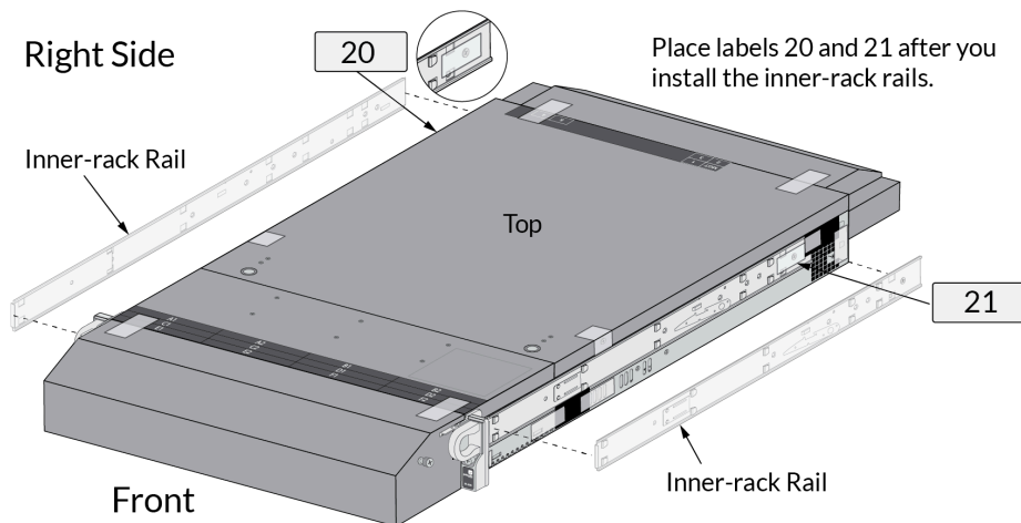
Figure 28 – M-600: Tamper Seals Location for Side Rails
