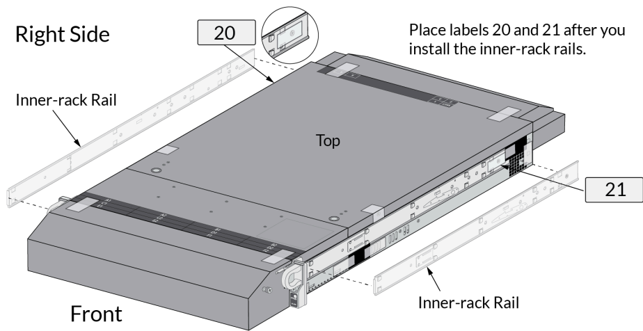
Figure 34 – M-700: Tamper Seals Location for Side Rails
