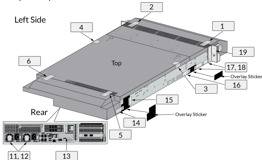
Figure 32 – M-700: Tamper Seal Locations (Top and Rear)
