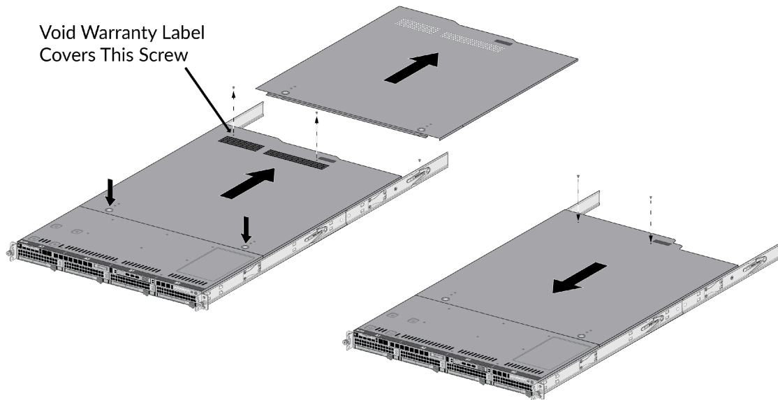
Figure 9 – M-200: Top Cover Replacement
