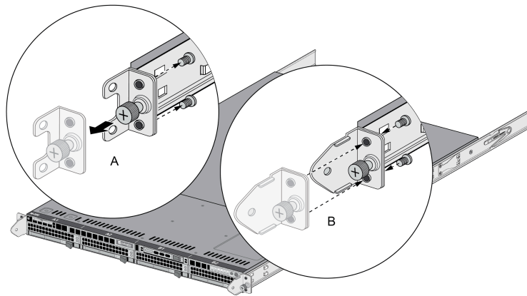
Figure 19 – M-300: Replacing Front Rack-Mount Brackets
