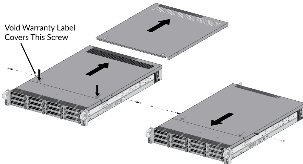
Figure 29 – M-700: Top Cover Replacement
