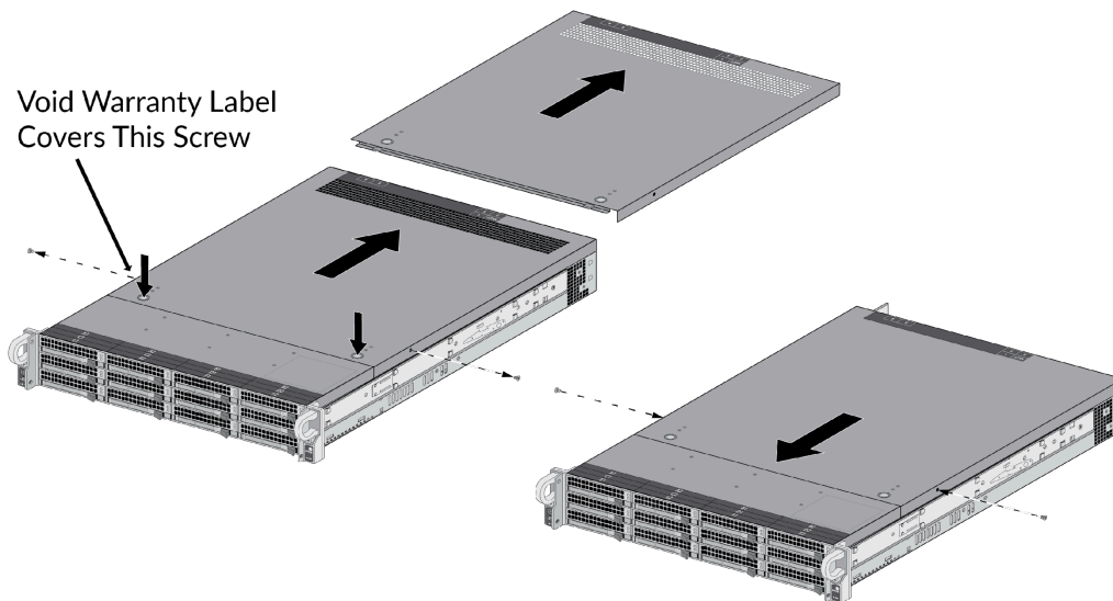
Figure 23 – M-600: Top Cover Replacement
