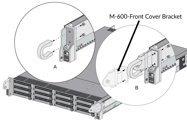
Figure 24 - M-600: Front Cover Bracket
