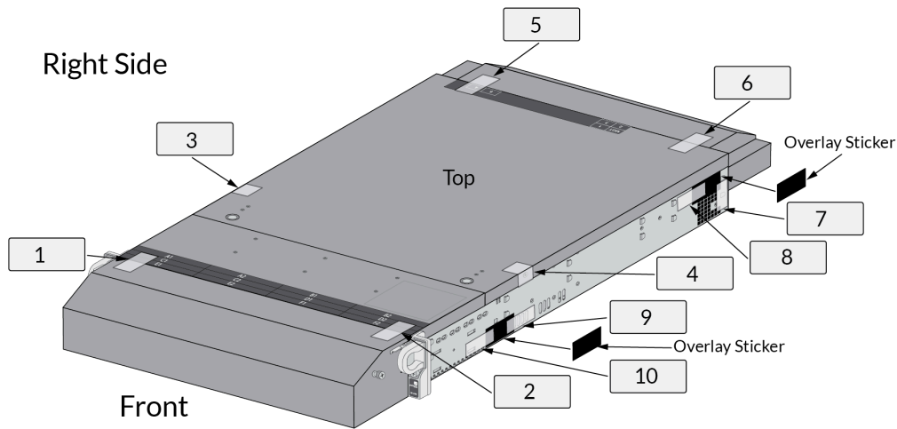
Figure 27 – M-600: Tamper Seal Locations (Top and Front)
