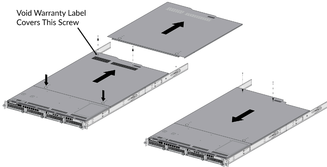
Figure 16 - M-300: Top Cover Replacement
