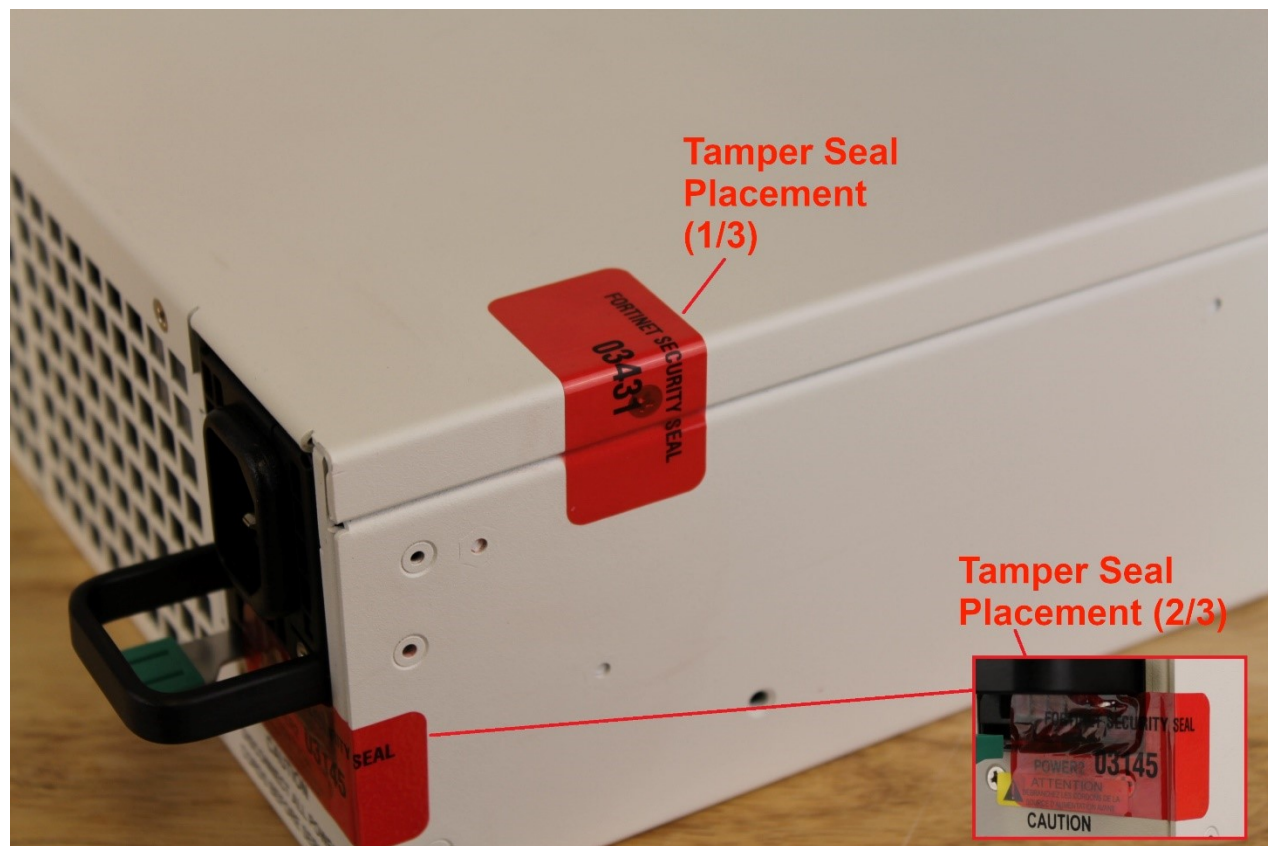
Figure 5 - FortiGate-3401E and 3601E external enclosure seal, back, left side
