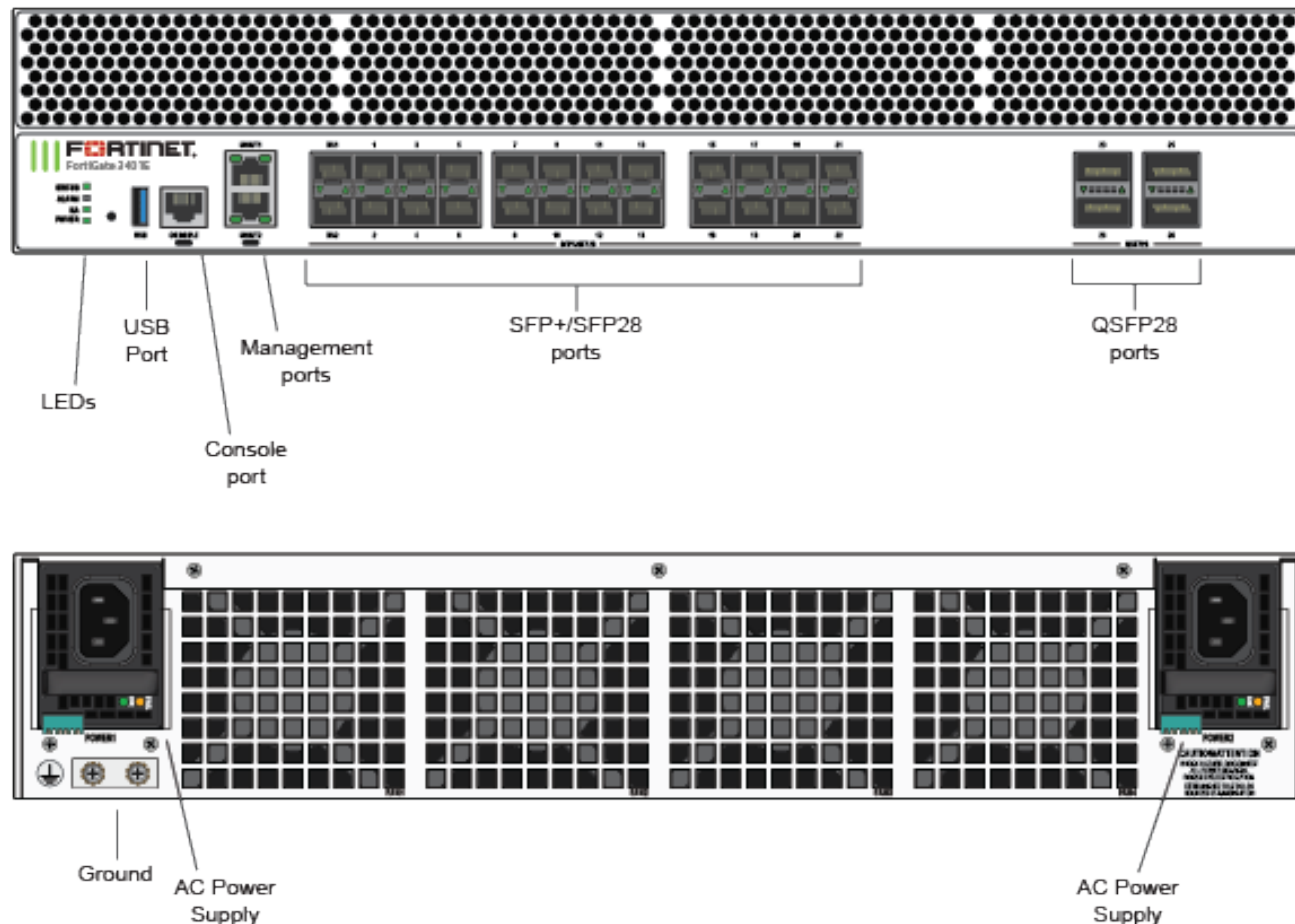
Figure 1 - FortiGate-3401E Front and Rear Panels
