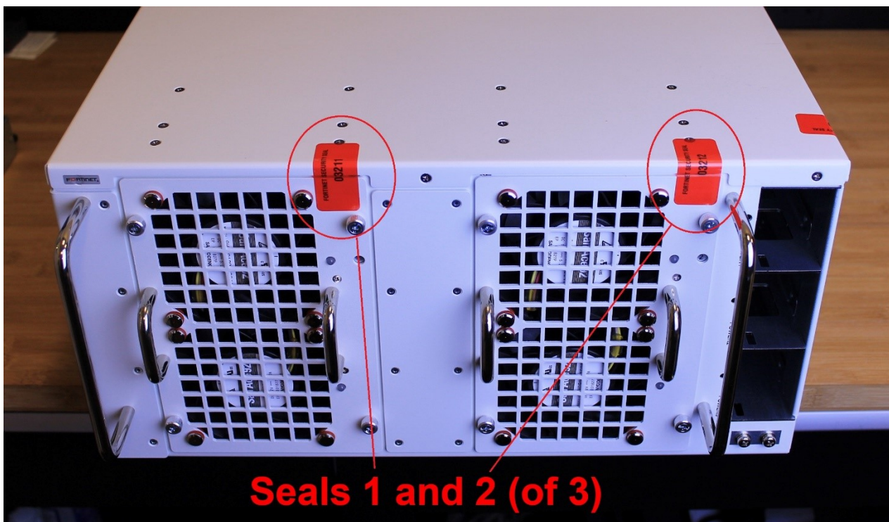
Figure 7 - FortiGate-3960E and 3980E external enclosure seals, top, back
