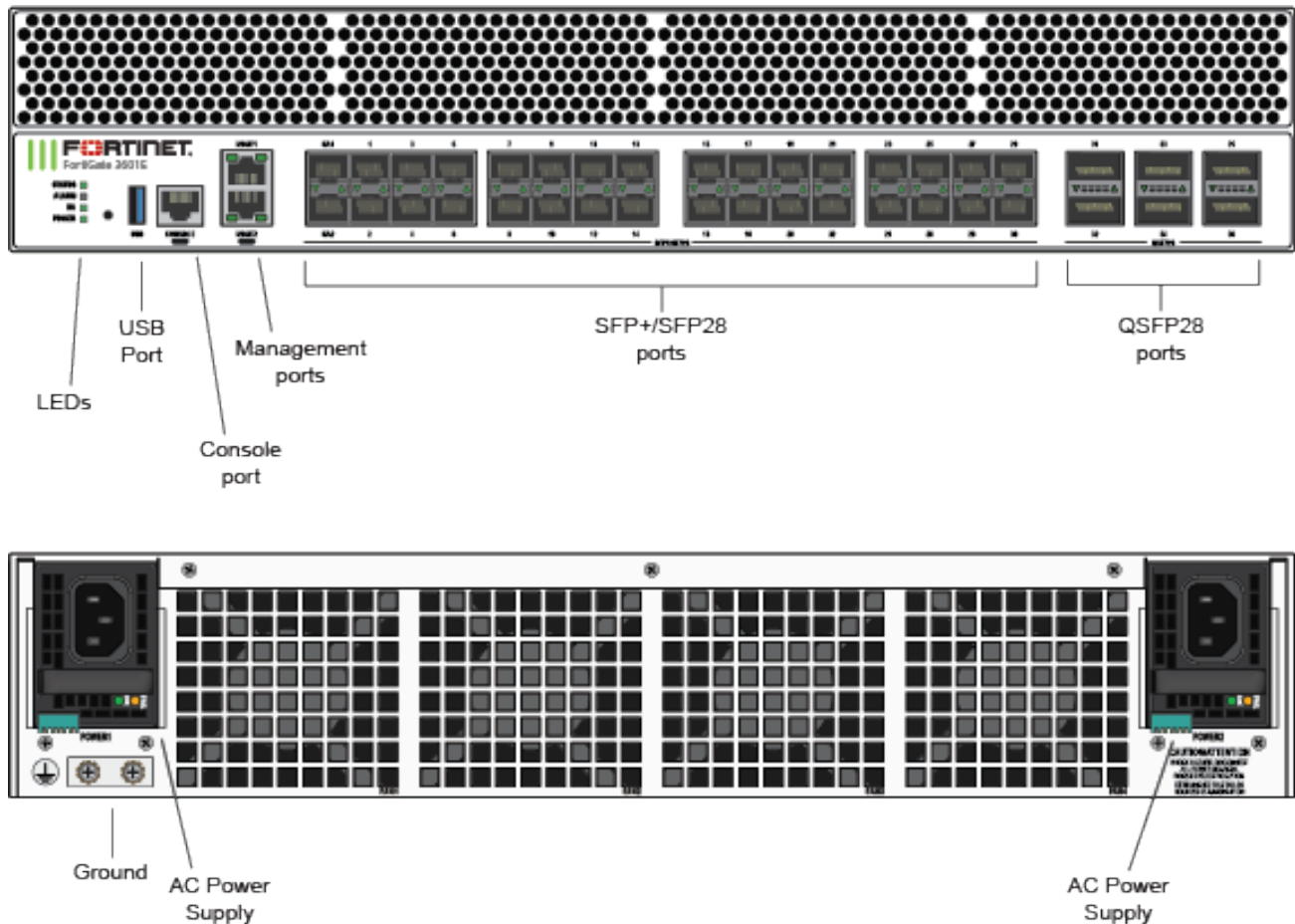
Figure 2 - FortiGate-3601E Front and Rear Panels
