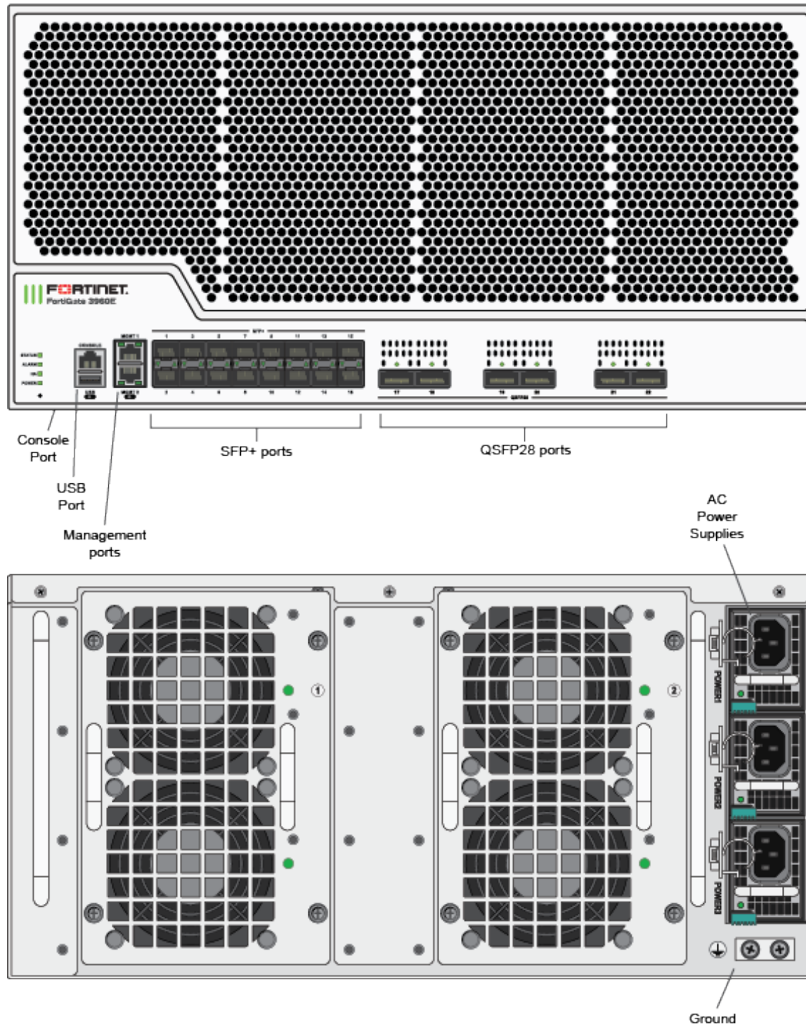
Figure 3 - FortiGate-3960E Front and Rear Panels
