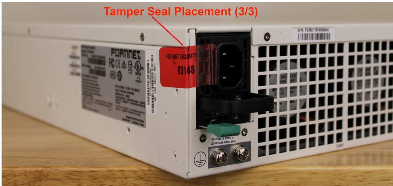
Figure 6 - FortiGate-3401E and 3601E external enclosure seal, back, right side
