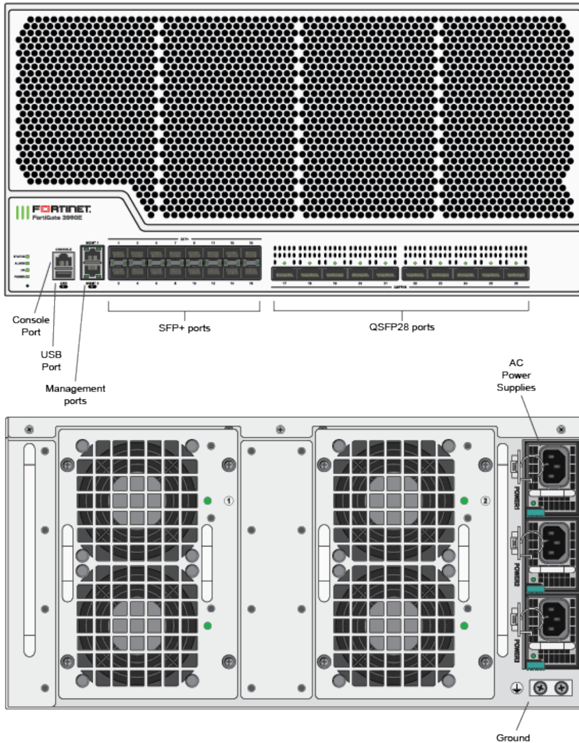
Figure 4 - FortiGate-3980E Front and Rear Panels
