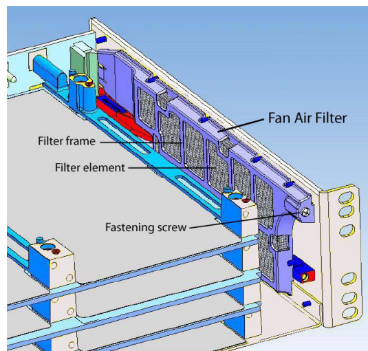
Figure 4 Location of Fan Air Filter in INUe
