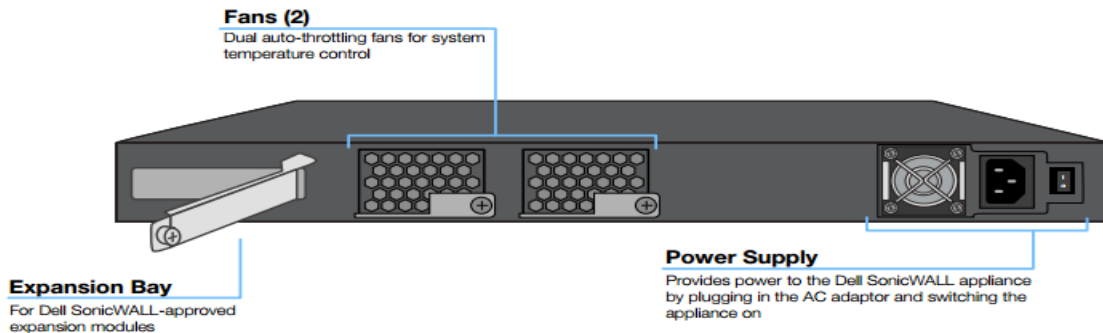
Figure 4 - NSA 6600 Back Panel
