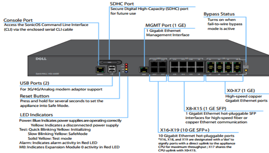
Figure 3 – NSA 6600 Front Panel
