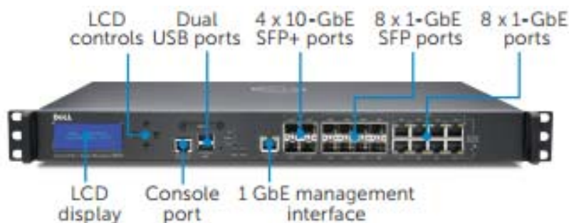
Figure 1 – Super Massive Front Panel
