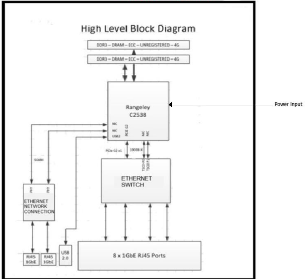
Figure 9: Block Diagram of the Trellix Intrusion Prevention System Sensor NS3100 and NS3200
