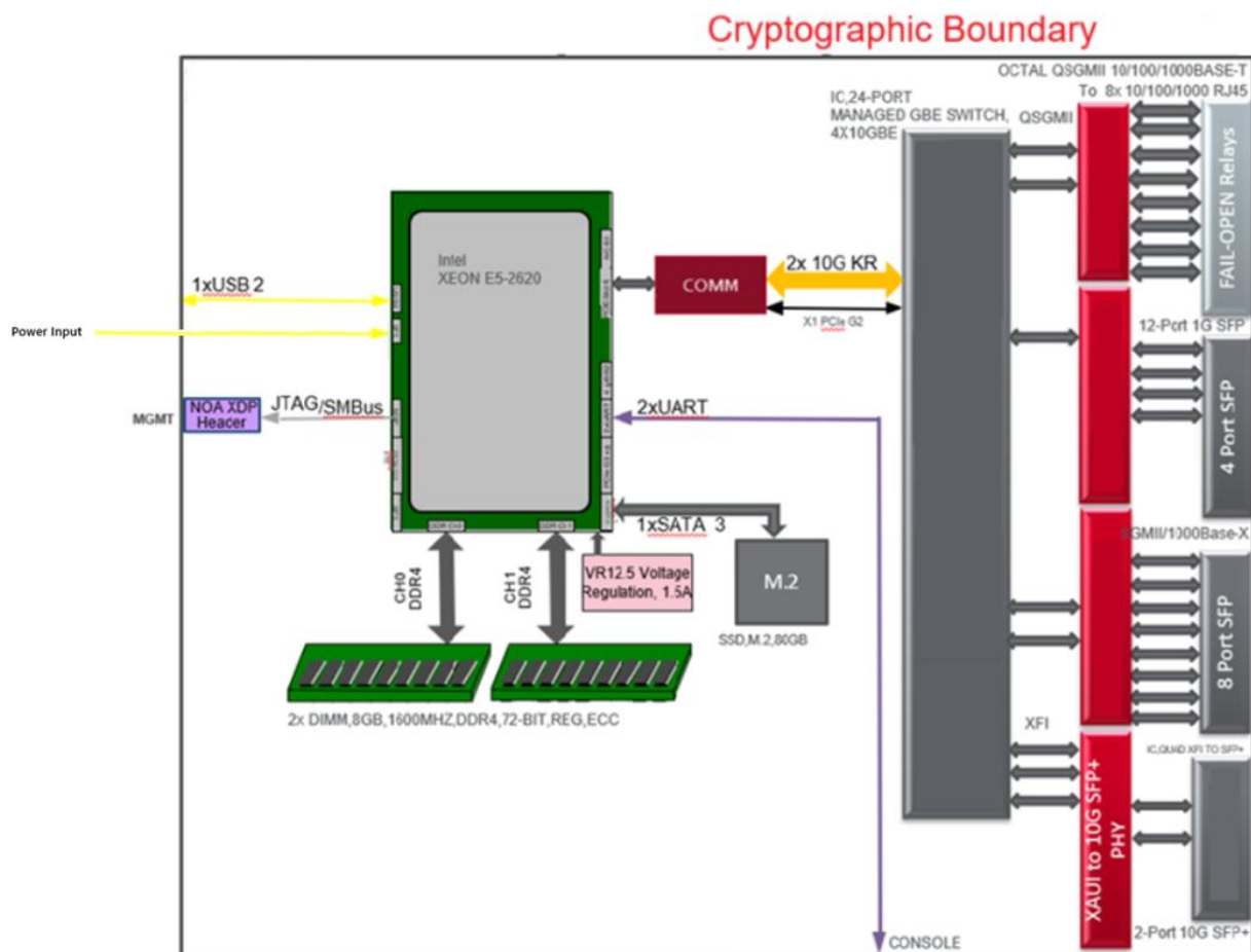
Figure 10: Block Diagram of the Trellix Intrusion Prevention System Sensor NS5100 and NS5200
