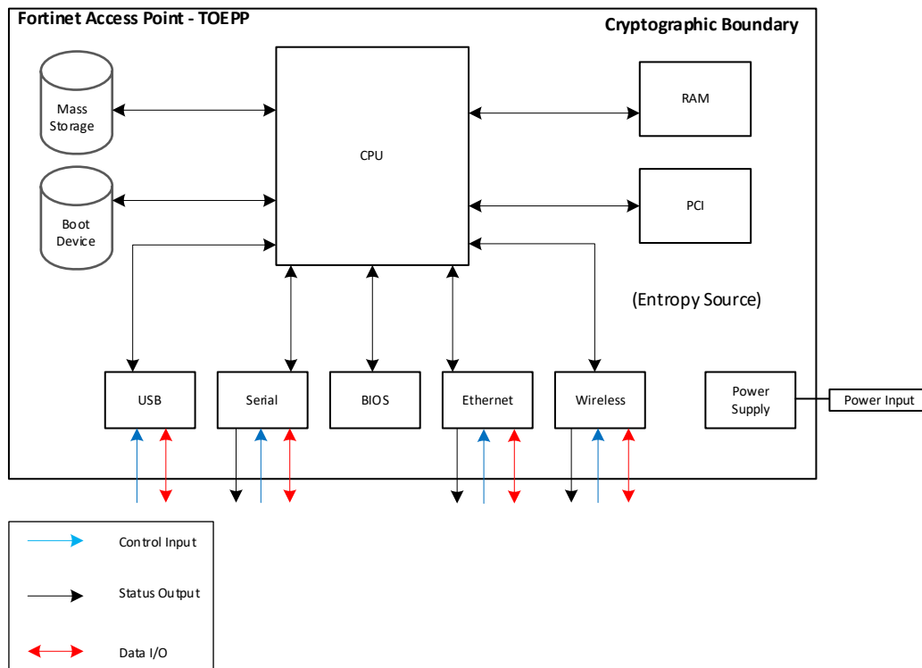
Figure 1 – Cryptographic Boundary and TOEPP.
