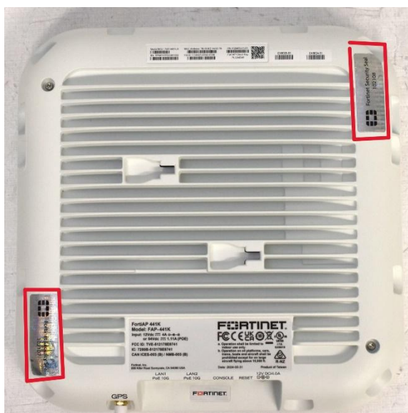
Figure 6 - FortiAP-441K seal placement.
