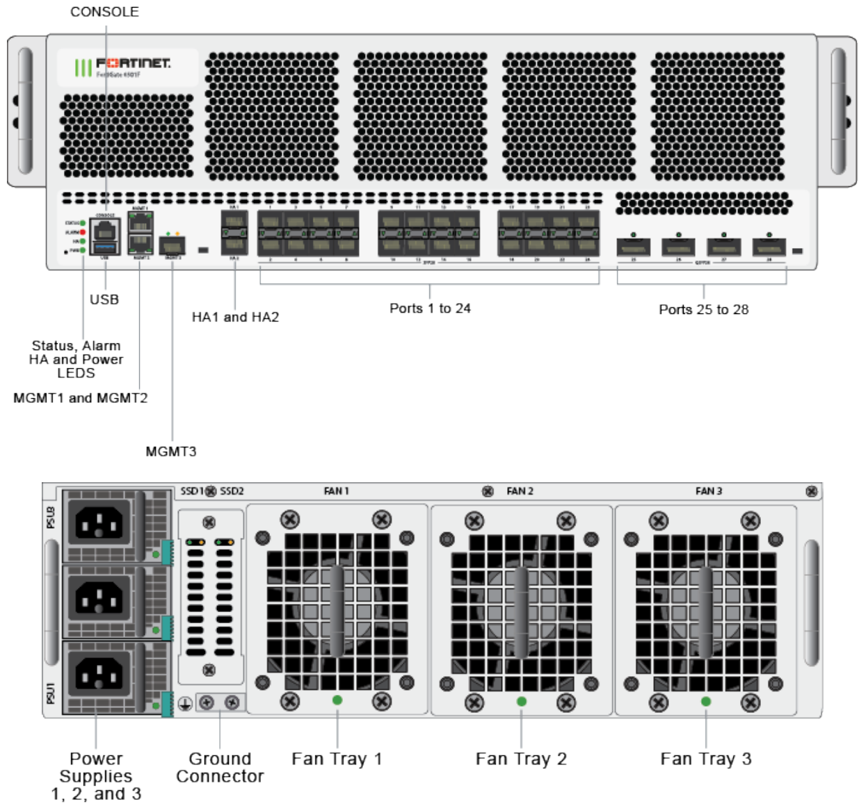
Figure 1 - FortiGate-6300F/6301F and 6500F/6501F Front and Rear Panels
