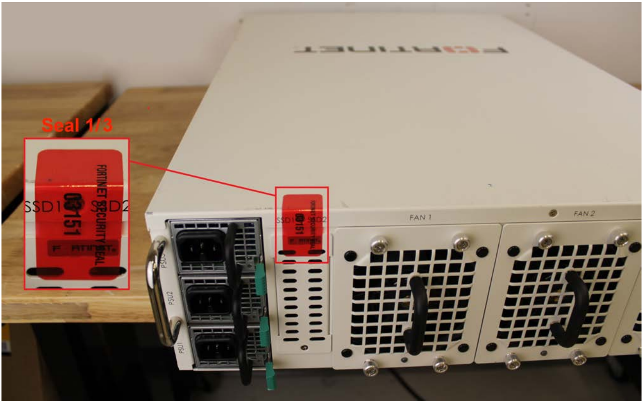
Figure 2 - FortiGate-6300F/6301F/6500F/6501F external enclosure seal 1, top, rear
