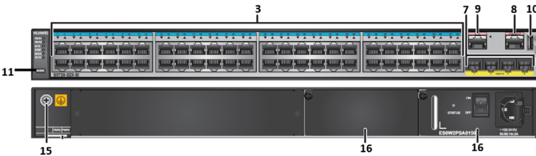
Figure 3-15: S5720-52X-SI-AC Ports – Front Panel (Top) & Back Panel (Bottom)
