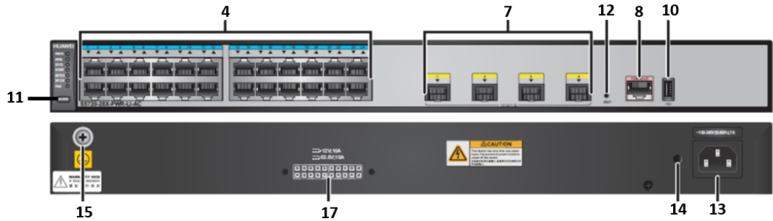
Figure 3-5: S5720-28X-PWR-LI-AC Ports – Front Panel (Top) & Back Panel (Bottom)
