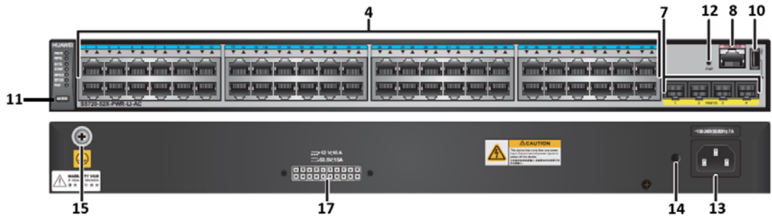
Figure 3-13: S5720-52X-PWR-LI-AC Ports – Front Panel (Top) & Back Panel (Bottom)
