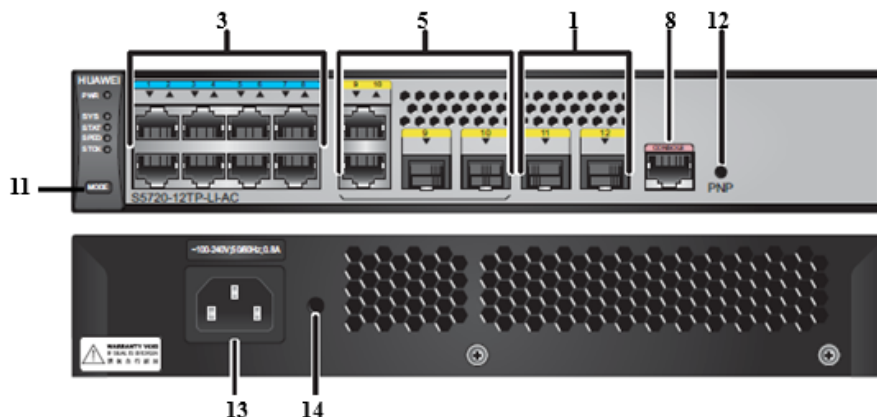
Figure 3-1: S5720-12TP-LI-AC Ports – Front Panel (Top) & Back Panel (Bottom)
