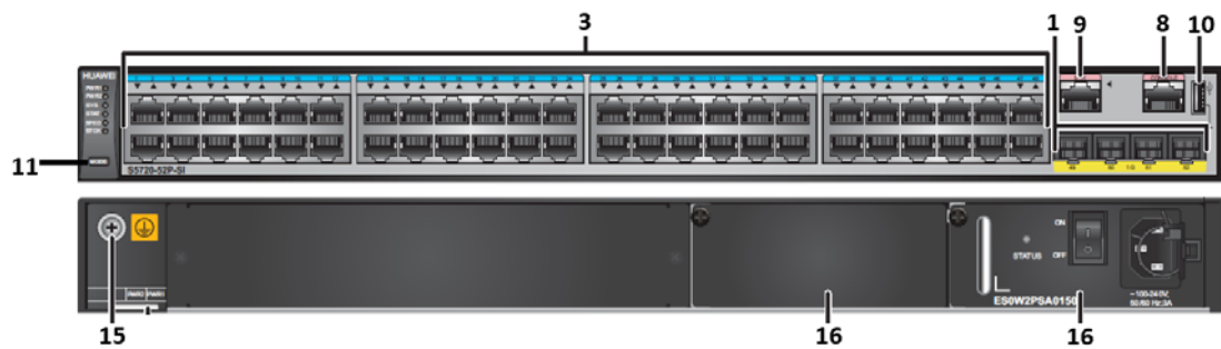
Figure 3-11: S5720-52P-SI-AC Ports – Front Panel (Top) & Back Panel (Bottom)
