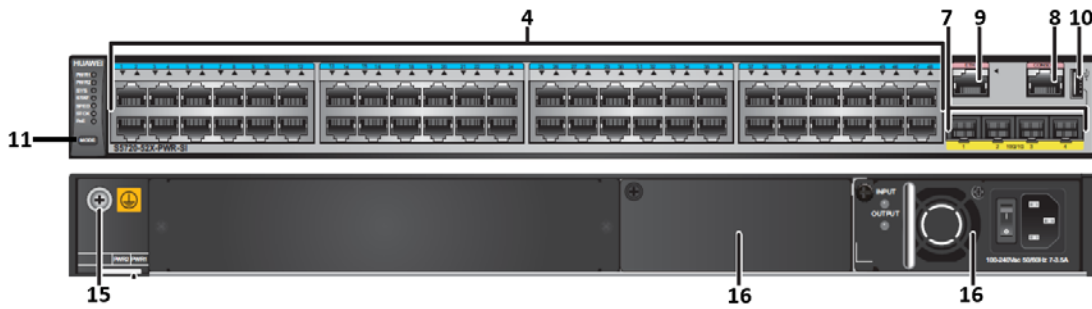
Figure 3-14: S5720-52X-PWR-SI-AC Ports – Front Panel (Top) & Back Panel (Bottom)
