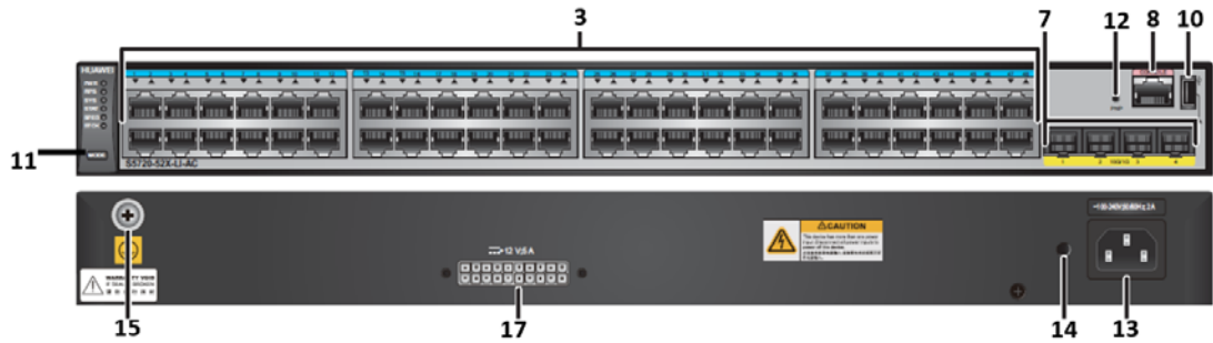
Figure 3-12: S5720-52X-LI-AC Ports – Front Panel (Top) & Back Panel (Bottom)
