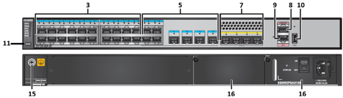
Figure 3-8: S5720-28X-SI-AC Ports – Front Panel (Top) & Back Panel (Bottom)
