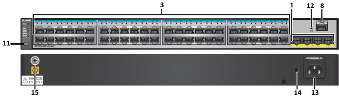
Figure 3-9: S5720-52P-LI-AC Ports – Front Panel (Top) & Back Panel (Bottom)
