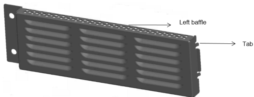
Figure 7-2: Insert the two tabs on the baffle into air vents on the left side of the switch.
