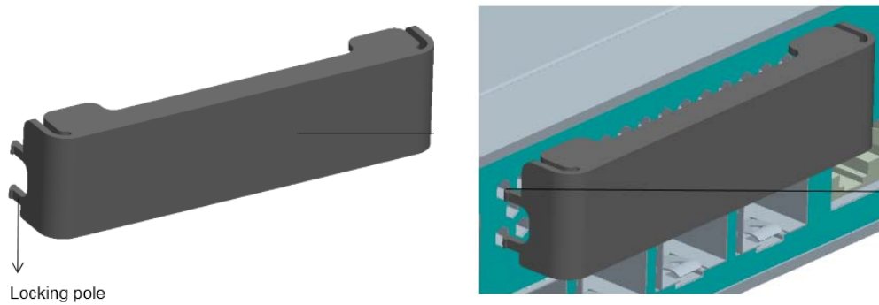
Figure 7-7: Take advantage of the plastic baffle’s elasticity to fit the locking poles of the baffle in air vents on the front panel.
