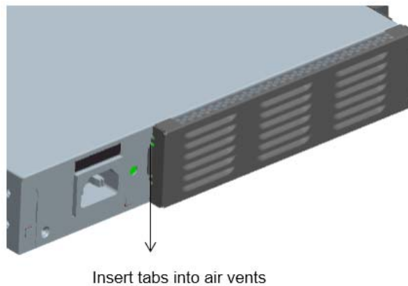
Figure 7-6: Gently push the baffle to fit the tabs in the air vents. Use two M4*10 screws to fix the baffles.
