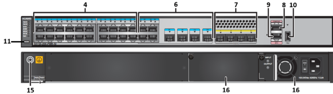
Figure 3-6: S5720-28X-PWR-SI-AC Ports – Front Panel (Top) & Back Panel (Bottom)
