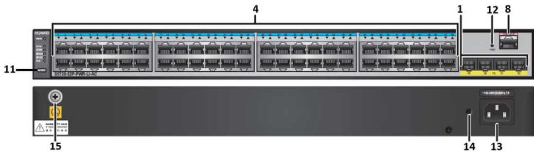
Figure 3-10: S5720-52P-PWR-LI-AC Ports – Front Panel (Top) & Back Panel (Bottom)
