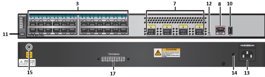
Figure 3-4: S5720-28X-LI-AC Ports – Front Panel (Top) & Back Panel (Bottom)
