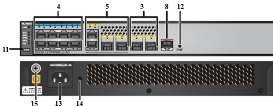
Figure 3-2: S5720-12TP-PWR-LI-AC Ports – Front Panel (Top) & Back Panel (Bottom)
