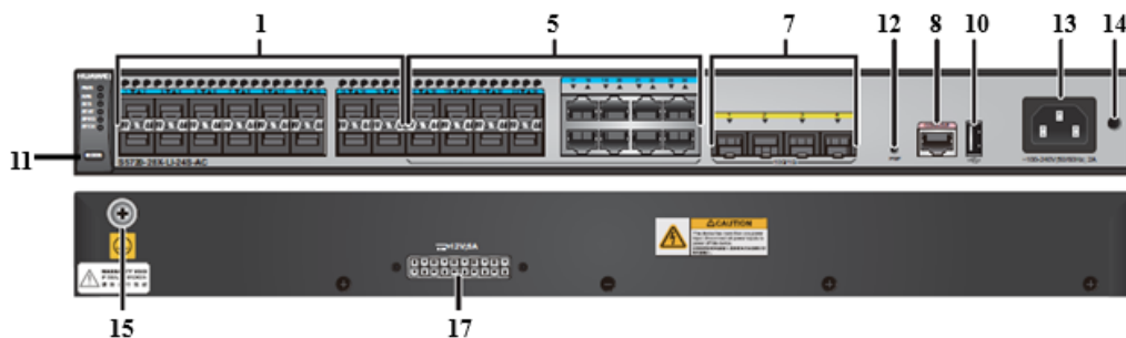
Figure 3-3: S5720-28X-LI-24S-AC Ports – Front Panel (Top) & Back Panel (Bottom)
