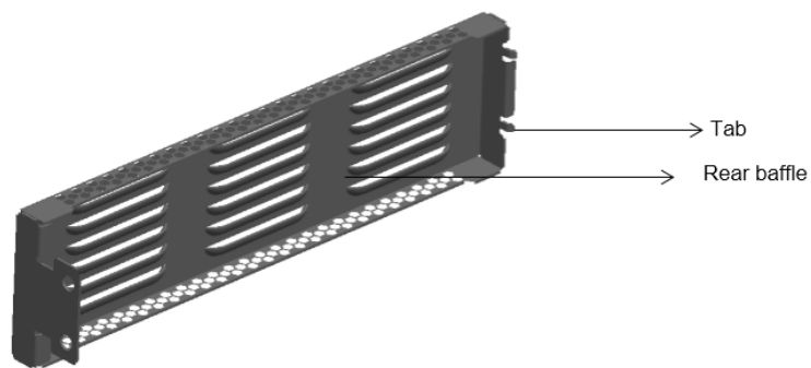
Figure 7-5: Insert the two tabs on the baffle into air vents on the rear of the switch.
