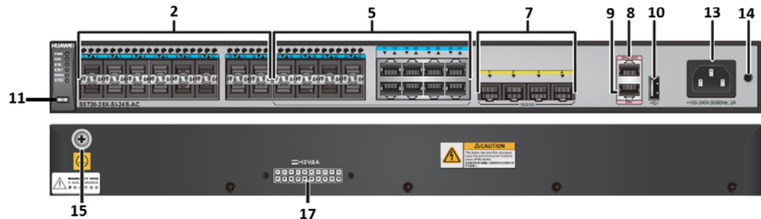
Figure 3-7: S5720-28X-SI-24S-AC Ports – Front Panel (Top) & Back Panel (Bottom)
