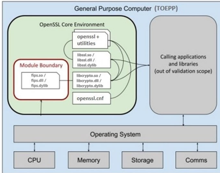
Figure 1: Splunk FIPS Provider (based on the OpenSSL FIPS Provider) Block Diagram
