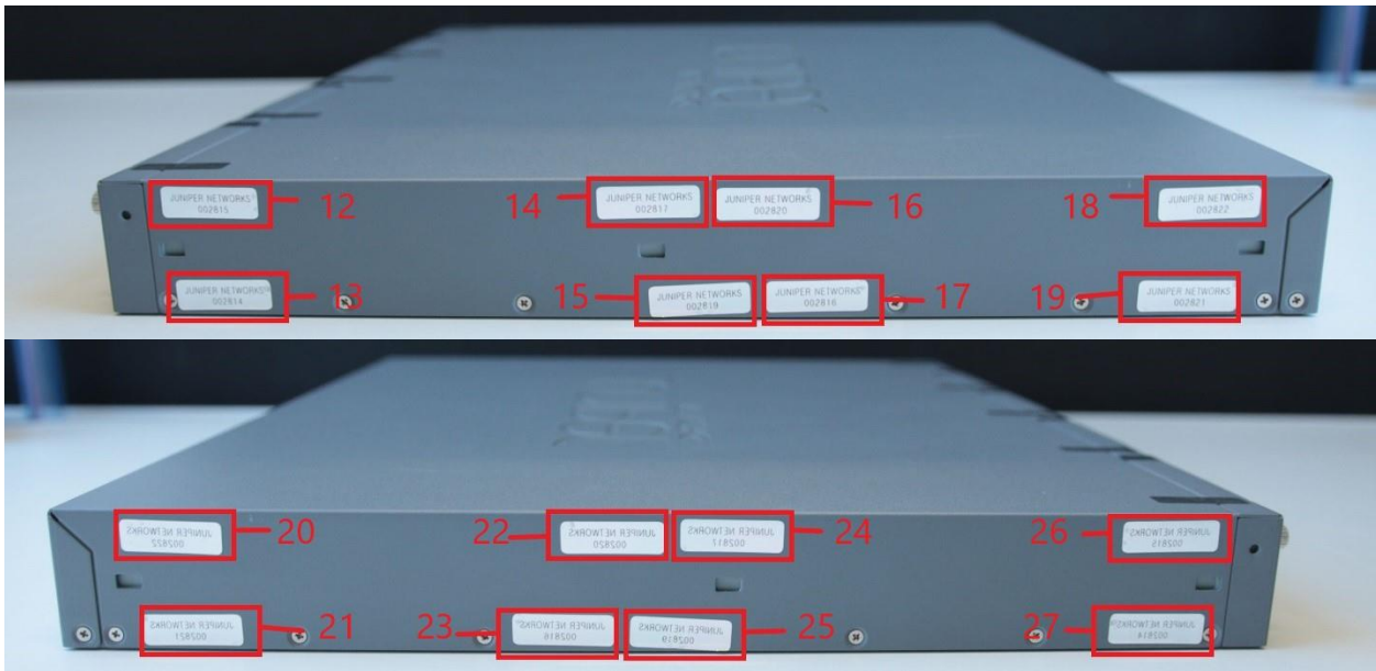
Figure 24 - SRX340/SRX345 Tamper-Evident Seal Placement (Right Side Panels, Eight on each side – Sixteen (16) Seals: TEL 12-27)
