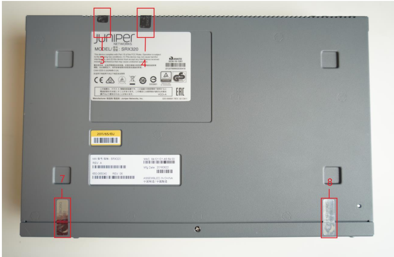
Figure 21 - SRX320 Tamper-Evident Seal Placement (Base Cover Screws (2) Seals TEL 7 & 8)
