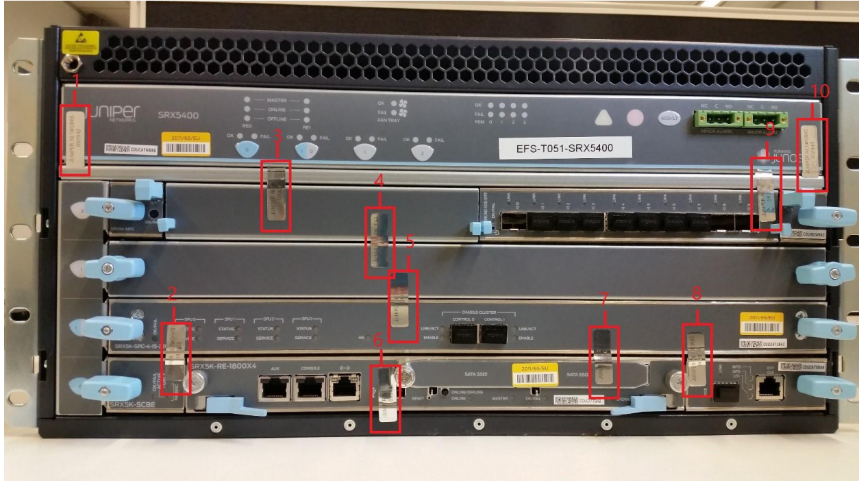
Figure 29 - SRX5400 Tamper-Evident Seal Locations (Front, Ten (10) Seals: TEL 1-10)
