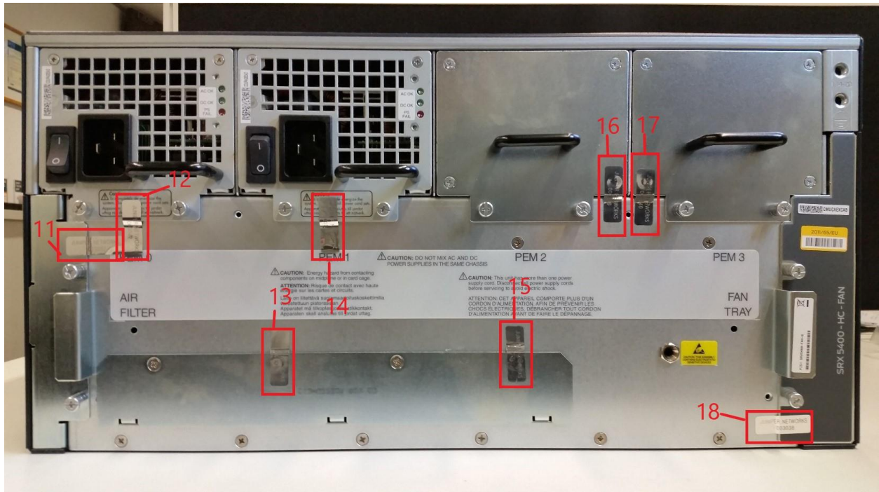
Figure 30 - SRX5400 Tamper-Evident Seal Locations (Rear, Eight (8) Seals: TEL 11-18)
