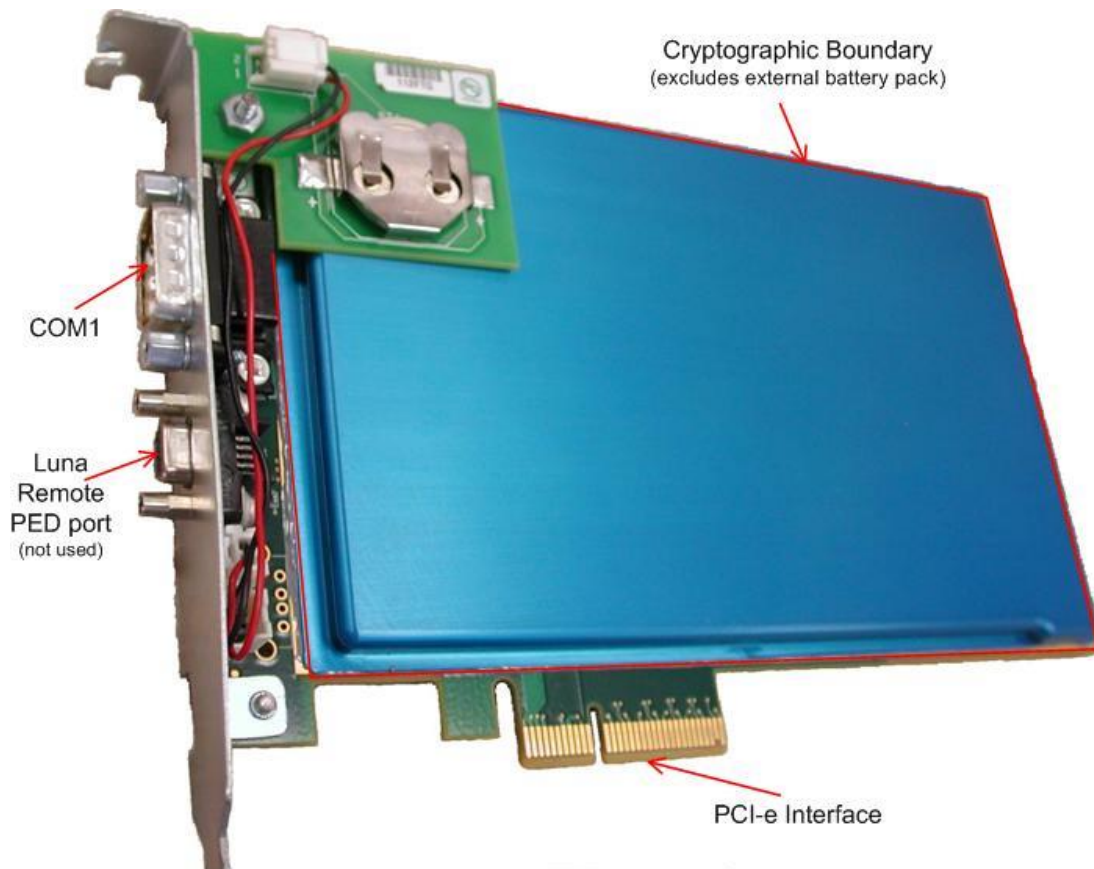
Figure 2-1 ProtectServer Internal Express Card
