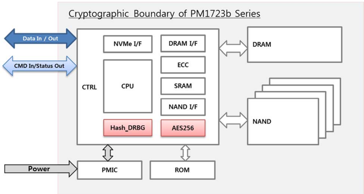
Exhibit 3 – Block Diagram for Samsung NVMe TCG Opal SSC SEDs PM1723b Series.
