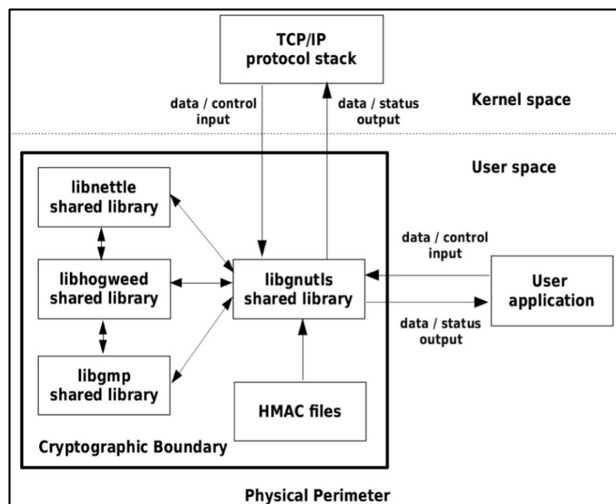
Figure 1: Block Diagram
